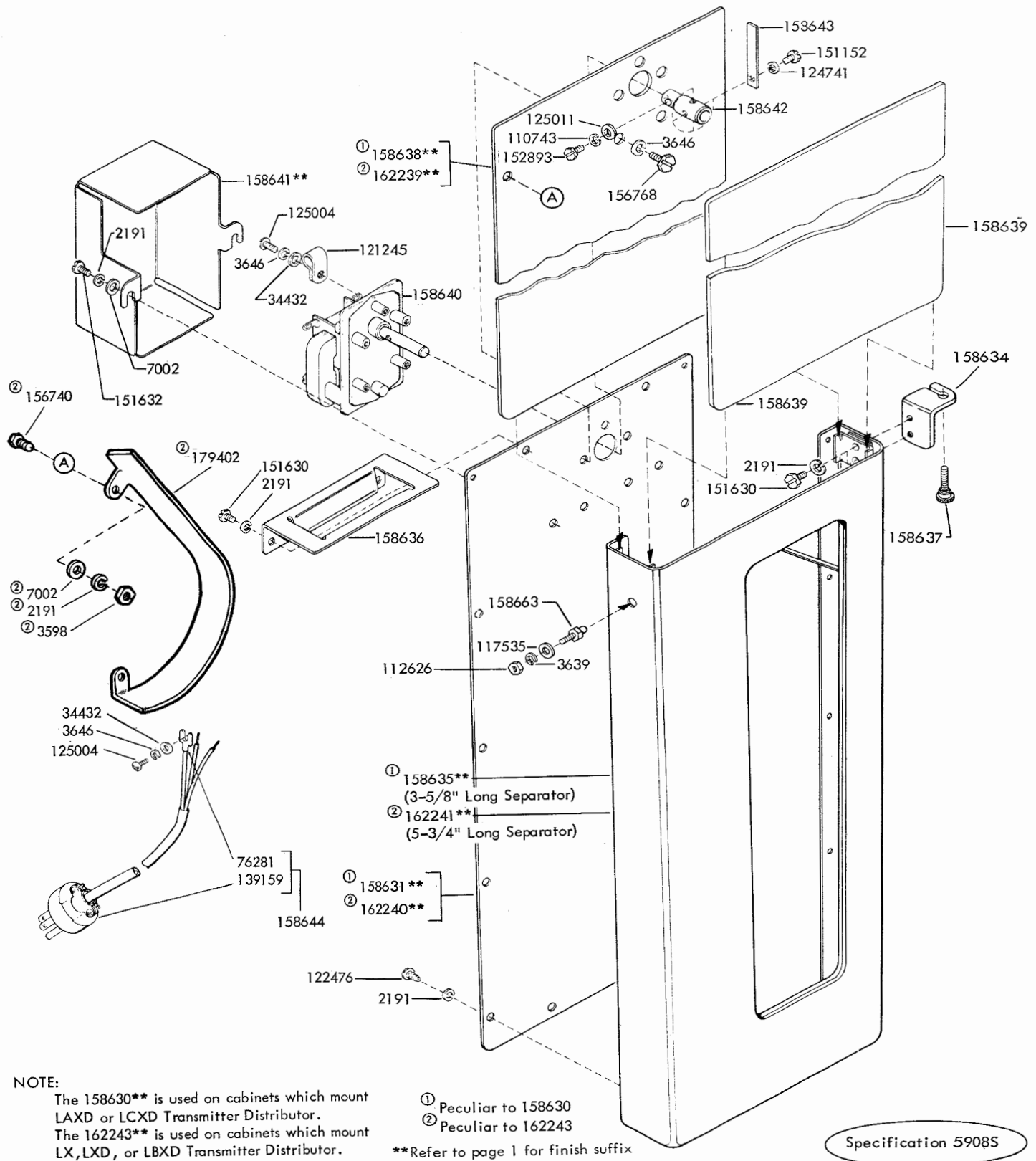
FIGURE 28. 158630** (FOR LAXD, LCXD) AND 162243** (FOR LX, LXD, AND LBXD) TAPE BIN ASSEMBLIES
