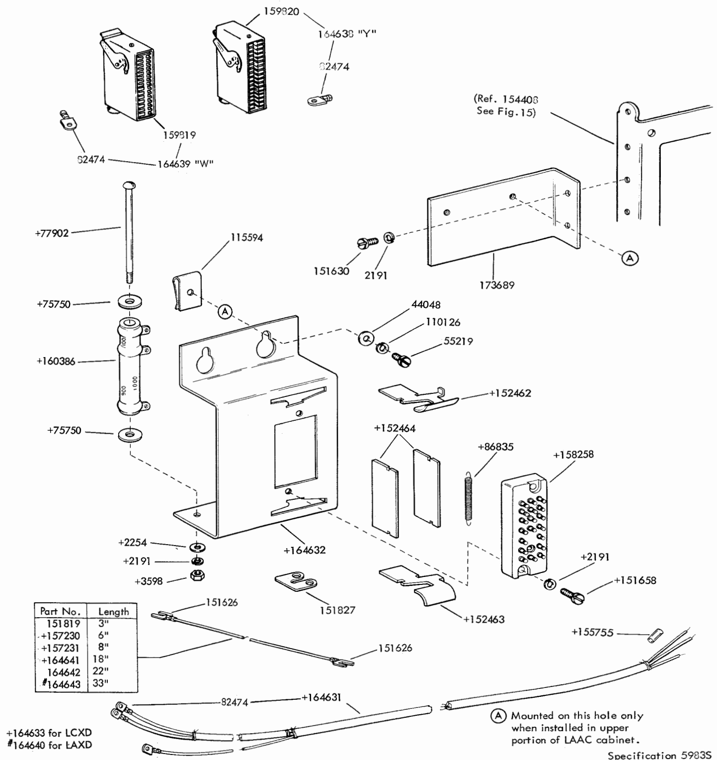
FIGURE 70. 164633 AND 164640 MODIFICATION KITS TO PERMIT LAXD3 AND LCXD1 TRANSMITTER DISTRIBUTORS TO OPERATE WITH LESU13 AND LESU15
