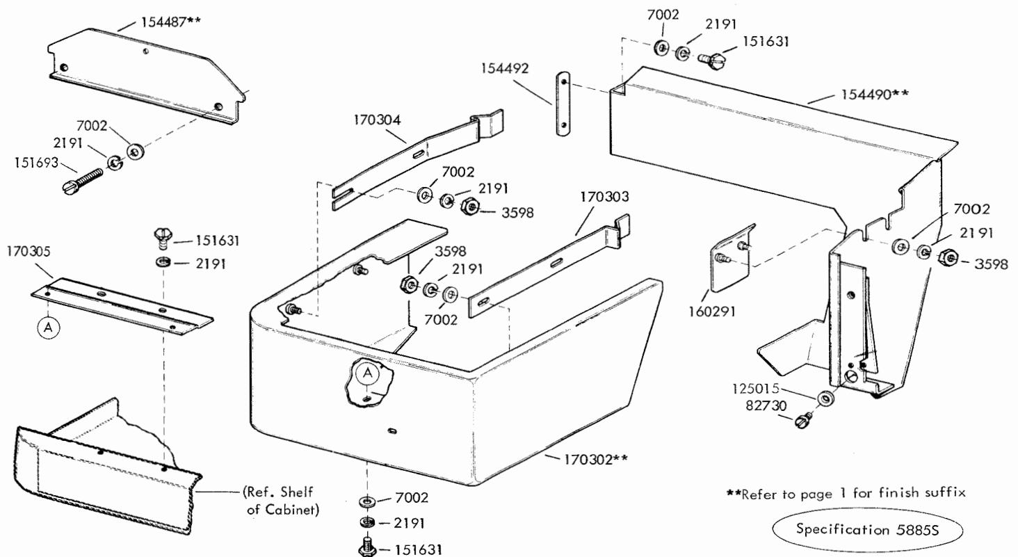
FIGURE 18. 170272** MODIFICATION KIT TO PROVIDE DUAL TRANSMITTER DISTRIBUTOR HOUSING
