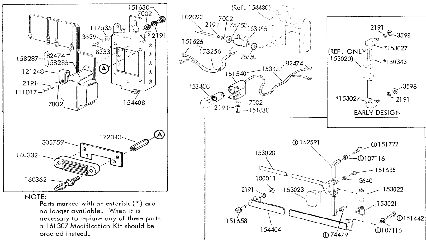
FIGURE 10. TRANSFORMER AND LINE GUIDE
