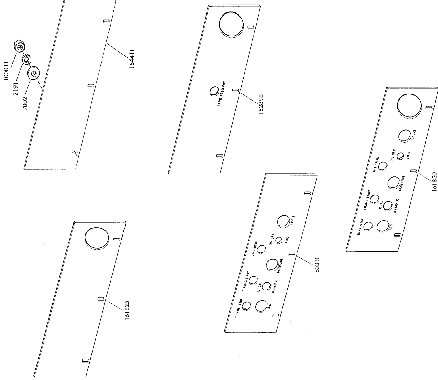
FIGURE 21. CONTROL PANELS
