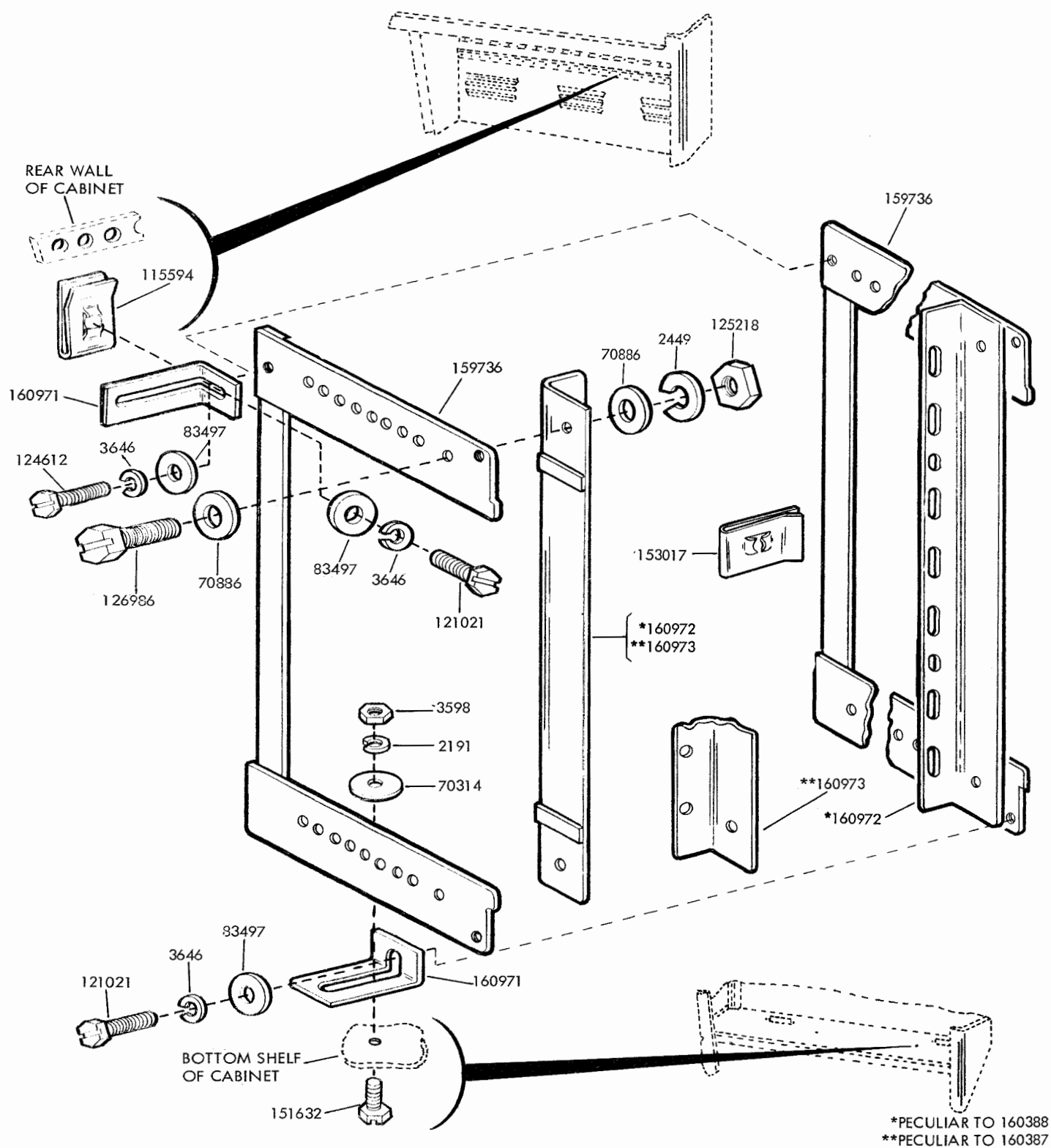
FIGURE 65. 160387 AND 160388 MODIFICATION KITS TO PROVIDE RELAY RACK BRACKETS
