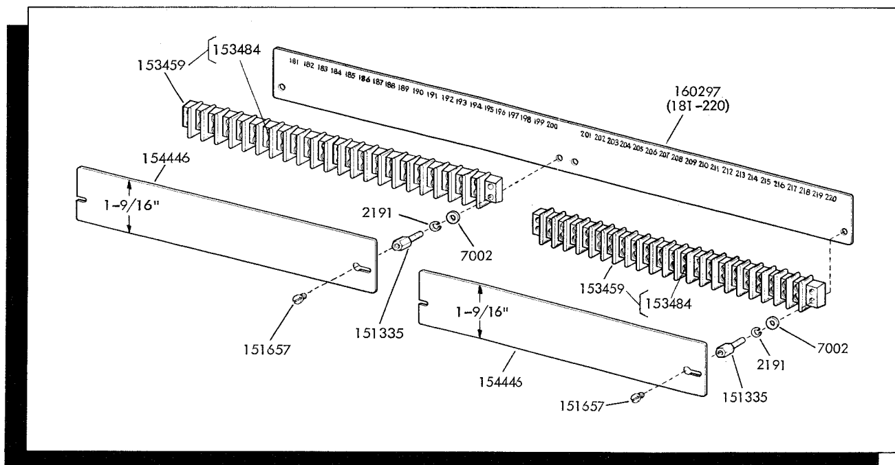
FIGURE 13. 159396 MODIFICATION KIT TO ADD AUXILIARY TERMINAL BLOCKS - TOP ROW LEFT REAR
