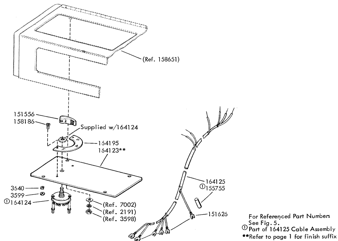
FIGURE 27. 164120** MODIFICATION KIT TO PROVIDE CONTROL PANEL
