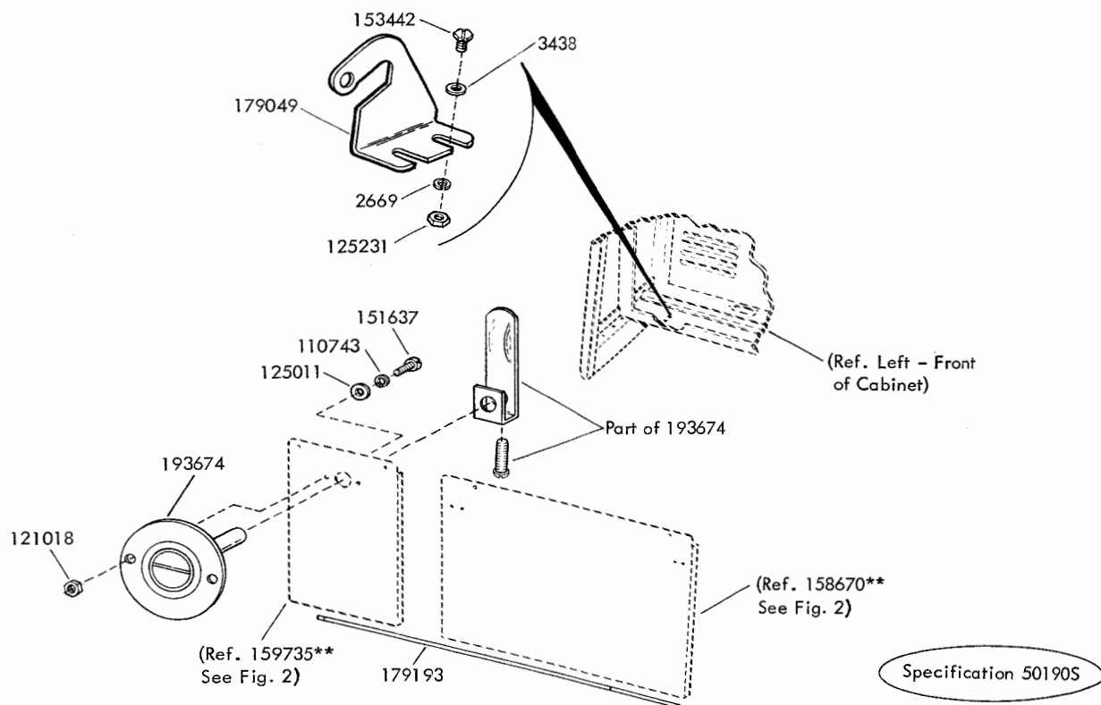
FIGURE 45. 193675 MODIFICATION KIT TO PROVIDE CABINET WITH TWO HINGED PANELS IN LOWER CAVITY
