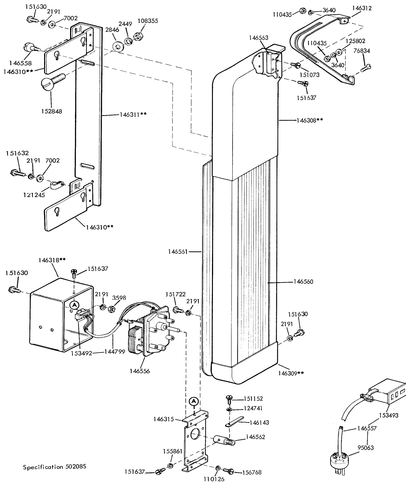
FIGURE 29. 145898** MODIFICATION KIT TO PROVIDE A TAPE BIN FOR STORED TAPE OF A MESSAGE IN TRANSMISSION
