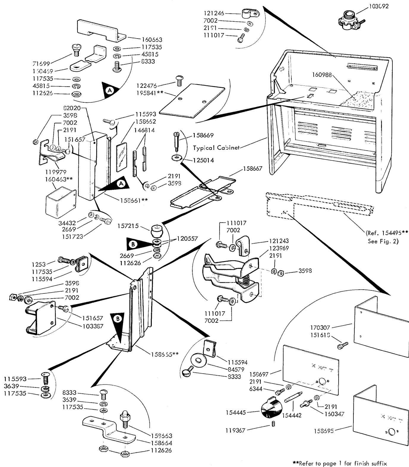
FIGURE 3. CABINET BASE COMMON PARTS (Continued)
