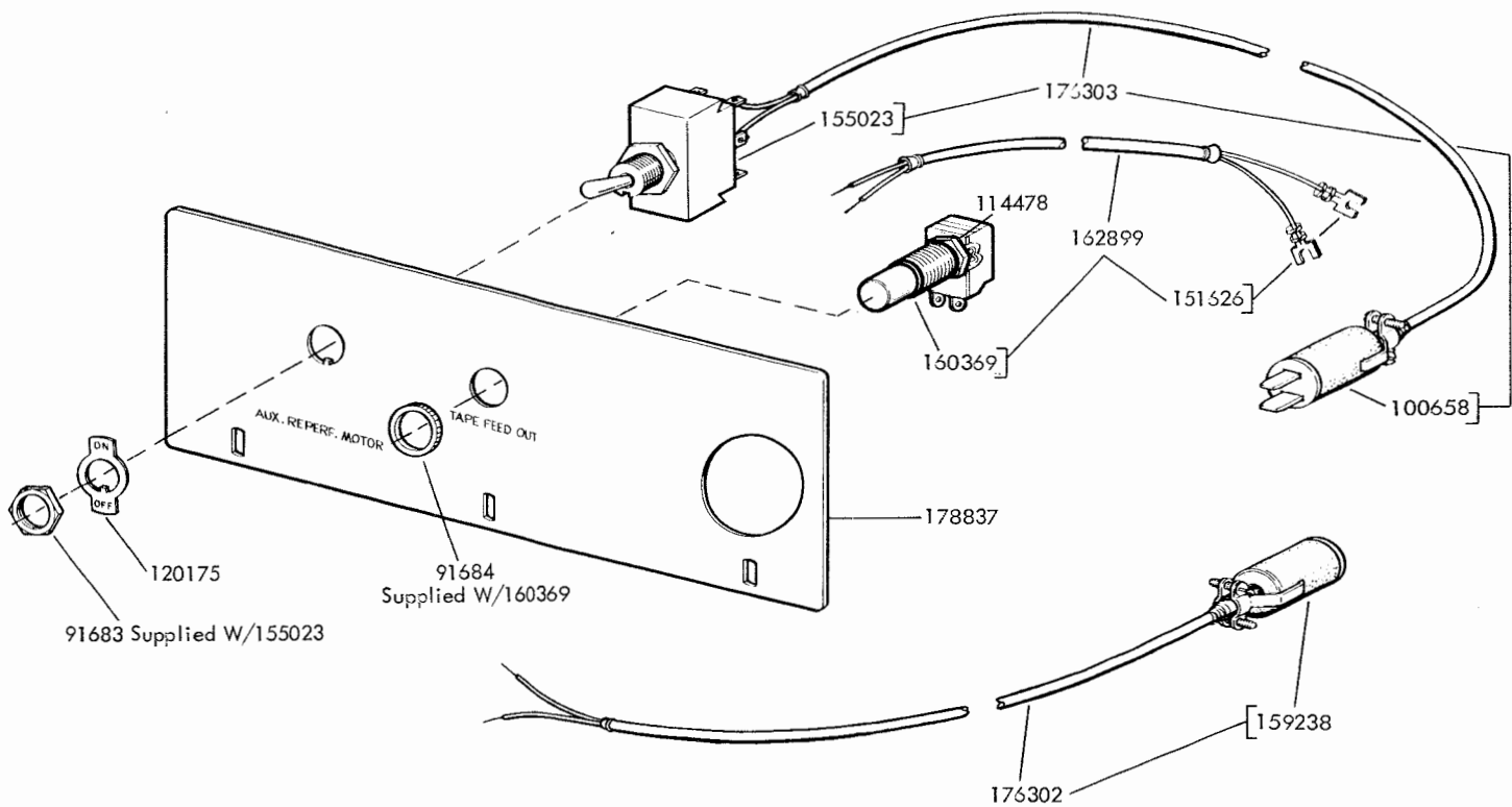
FIGURE 24. 178838 MODIFICATION KIT TO RELOCATE POWER SWITCH FROM AUXILIARY BASE TO OUTSIDE OF CABINET
