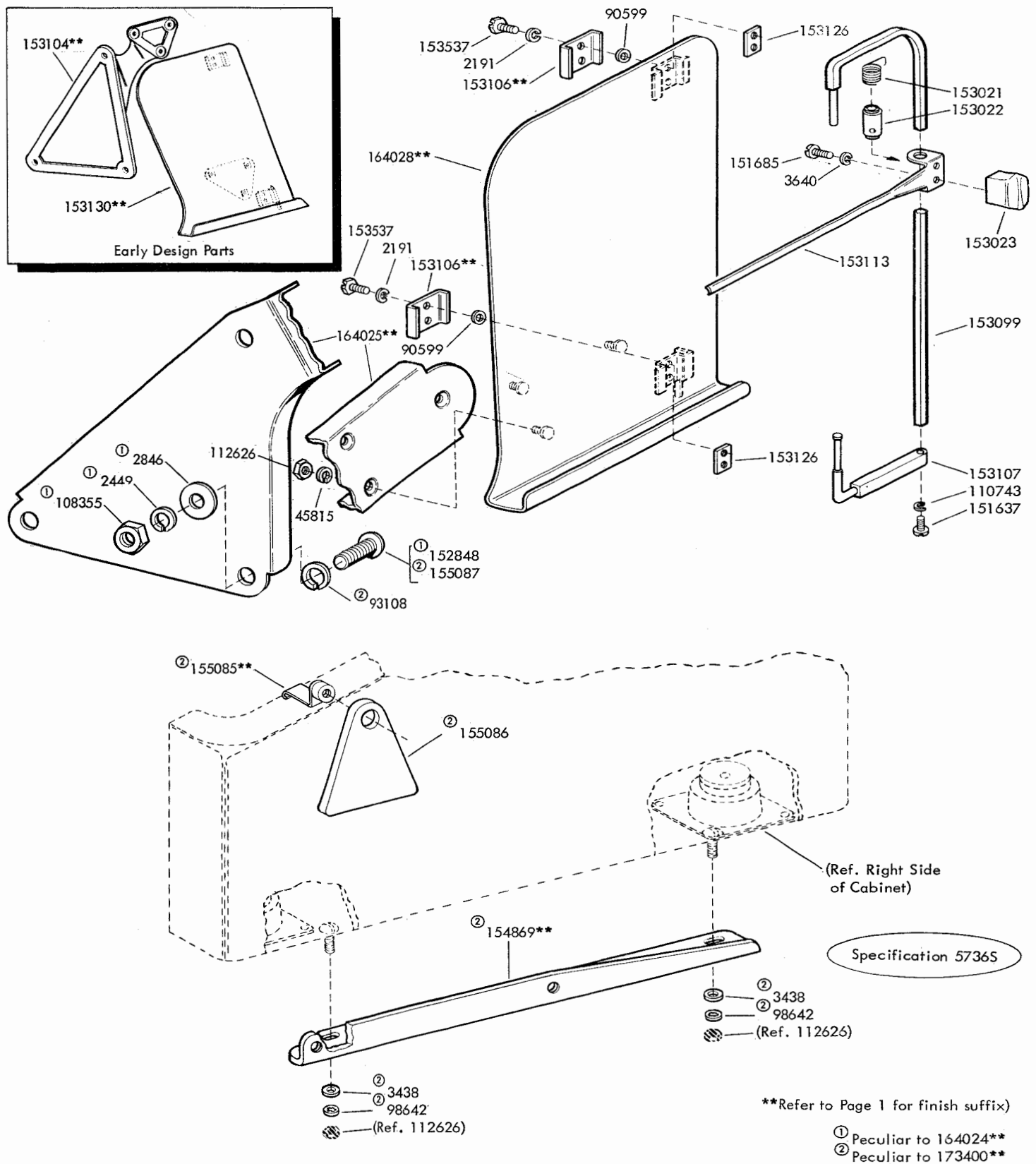
FIGURE 30. 164024** (FOR FLOOR MODEL) AND 173400** (FOR TABLE MODEL) MODIFICATION KITS TO PROVIDE OFFSET COPYHOLDER
