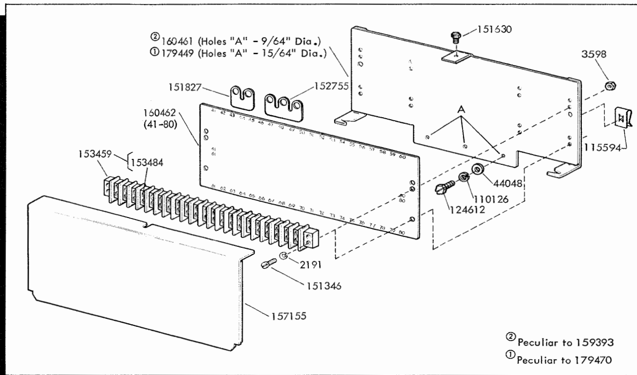
FIGURE 15. 159393 MODIFICATION KIT AND 179470 ASSEMBLY TO ADD AUXILIARY TERMINAL BLOCK - RIGHT SIDE
