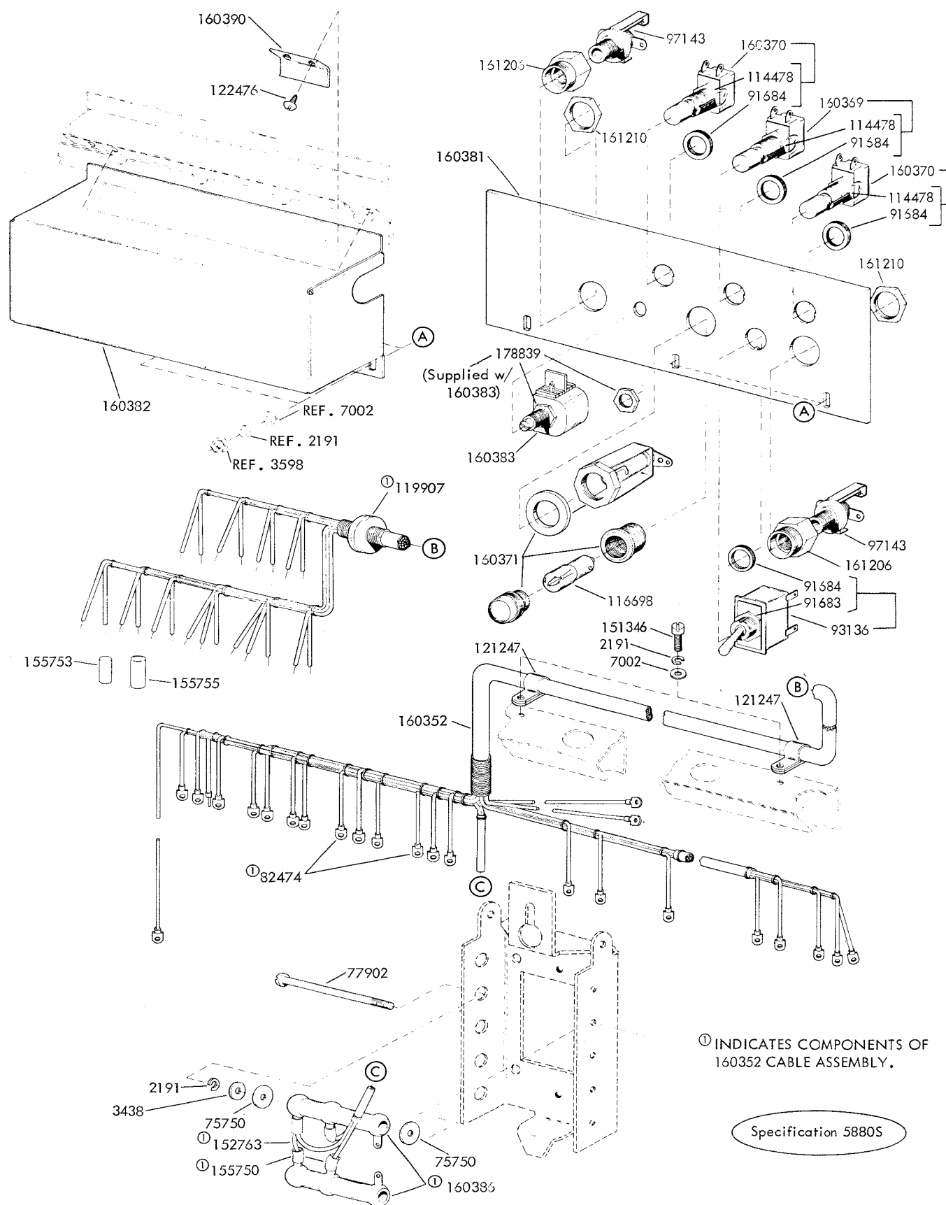
FIGURE 20. 160355 MODIFICATION KIT TO PROVIDE CONTROL PANEL FOR TRANSMITTER DISTRIBUTOR
