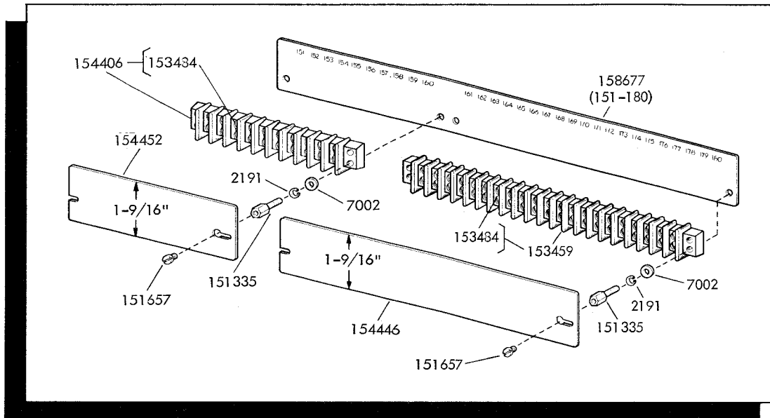
FIGURE 13. 159396 MODIFICATION KIT TO ADD AUXILIARY TERMINAL BLOCKS - TOP ROW LEFT REAR
