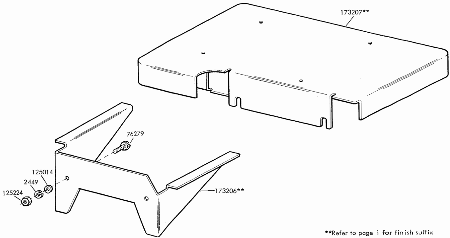
FIGURE 36. 173097** MODIFICATION KIT TO PROVIDE A MOUNTING SHELF FOR LEFT SIDE OF CABINET
