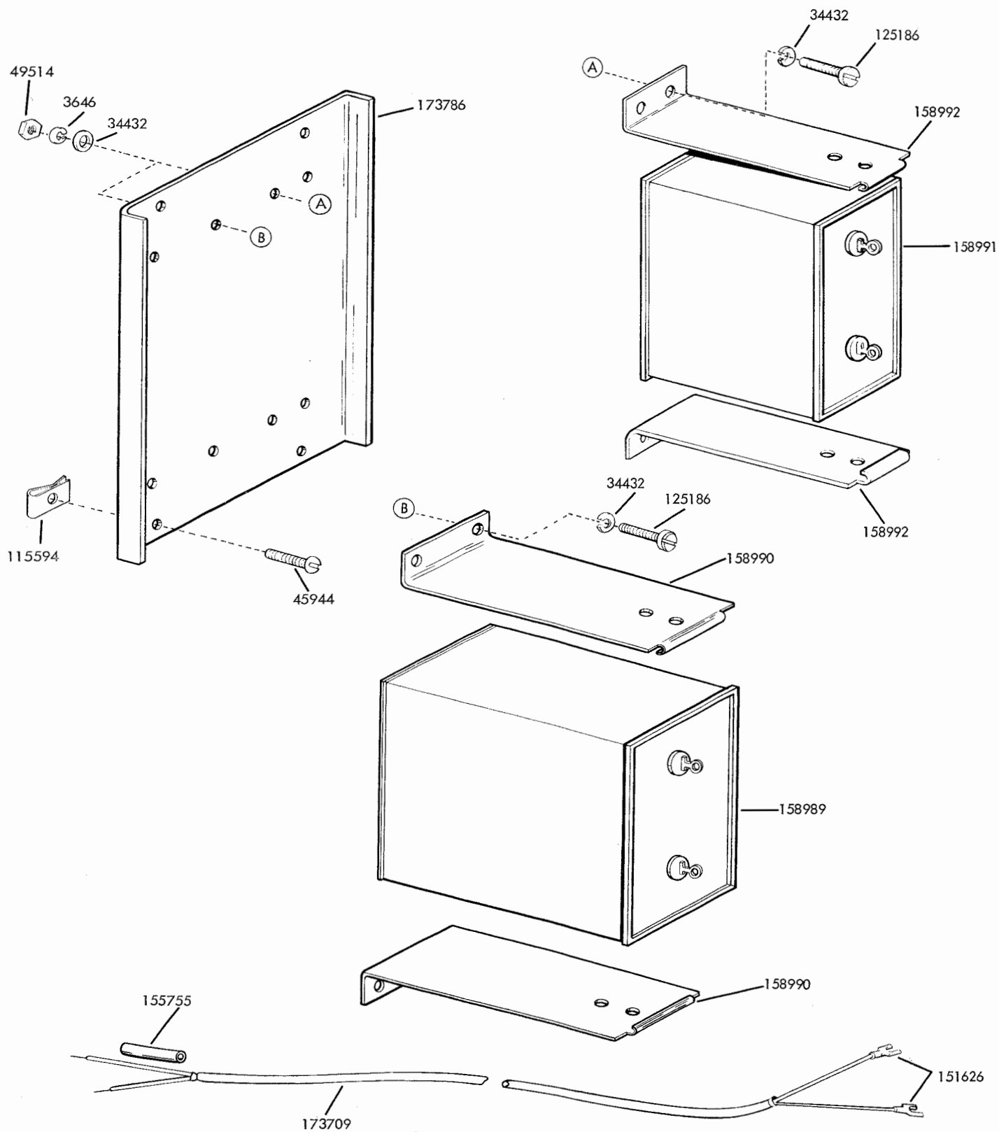
FIGURE 67. 173706 MODIFICATION KIT FOR POWER FACTOR CORRECTION IN CABINET (LAAC)
