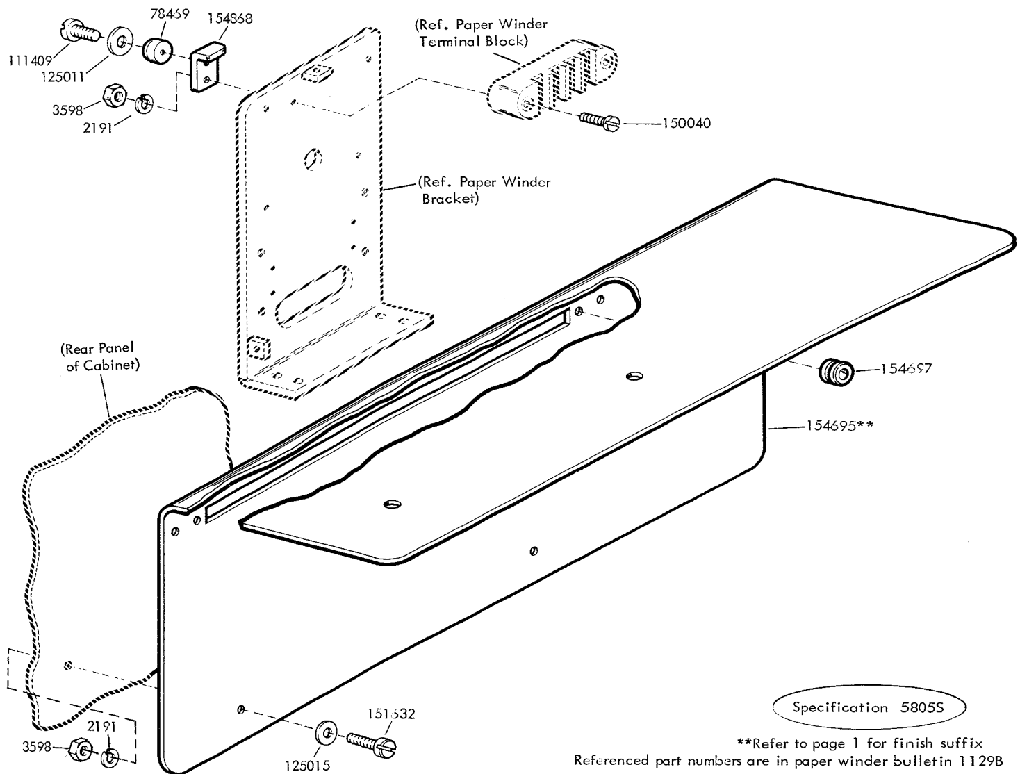
FIGURE 32. 153901** MODIFICATION KIT TO PROVIDE A SHELF FOR MOUNTING A PAPER WINDER TO CABINET
