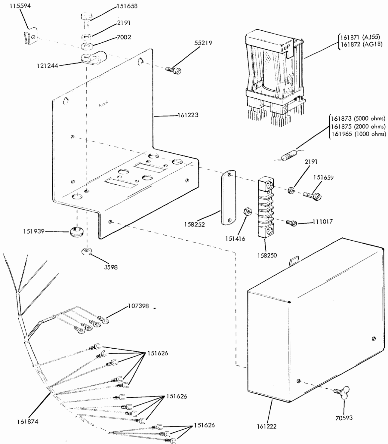
FIGURE 69. 161302 MODIFICATION KIT TO ADD AUTOMATIC CHARACTER FEED-OUT CIRCUIT TO AN ASR SET
