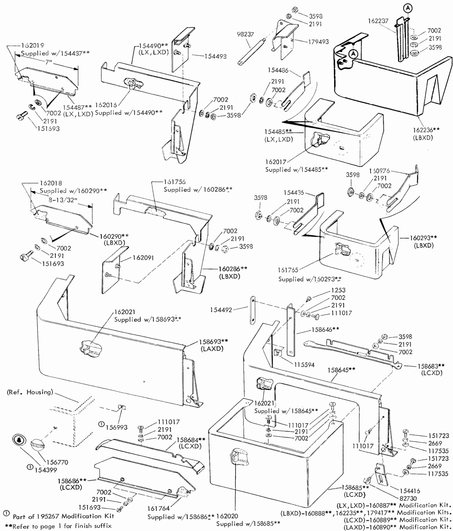
FIGURE 17. TRANSMITTER AND TRANSMITTER DISTRIBUTOR HOUSINGS
