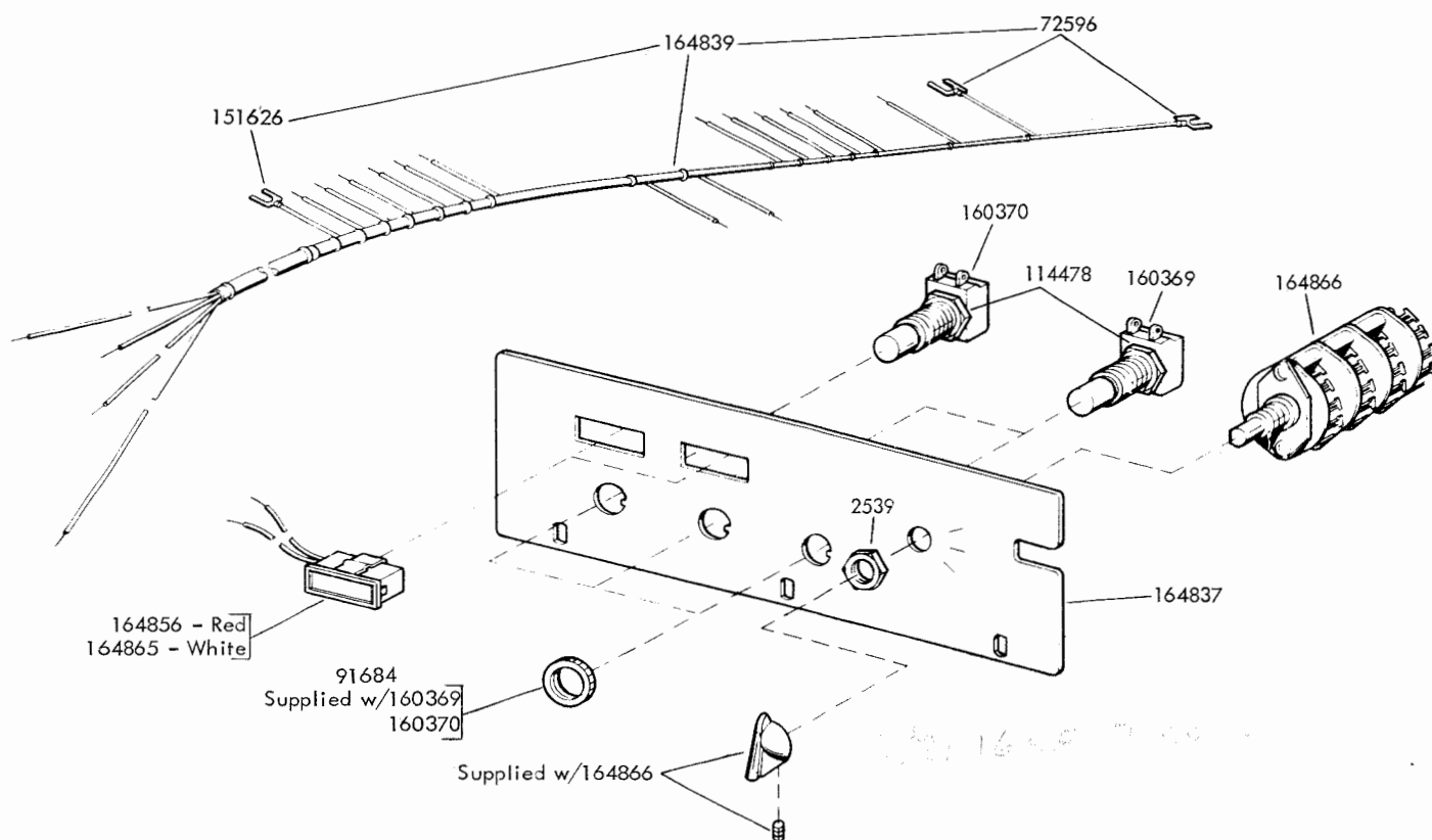
FIGURE 23. 164838 CONTROL PANEL ASSEMBLY
