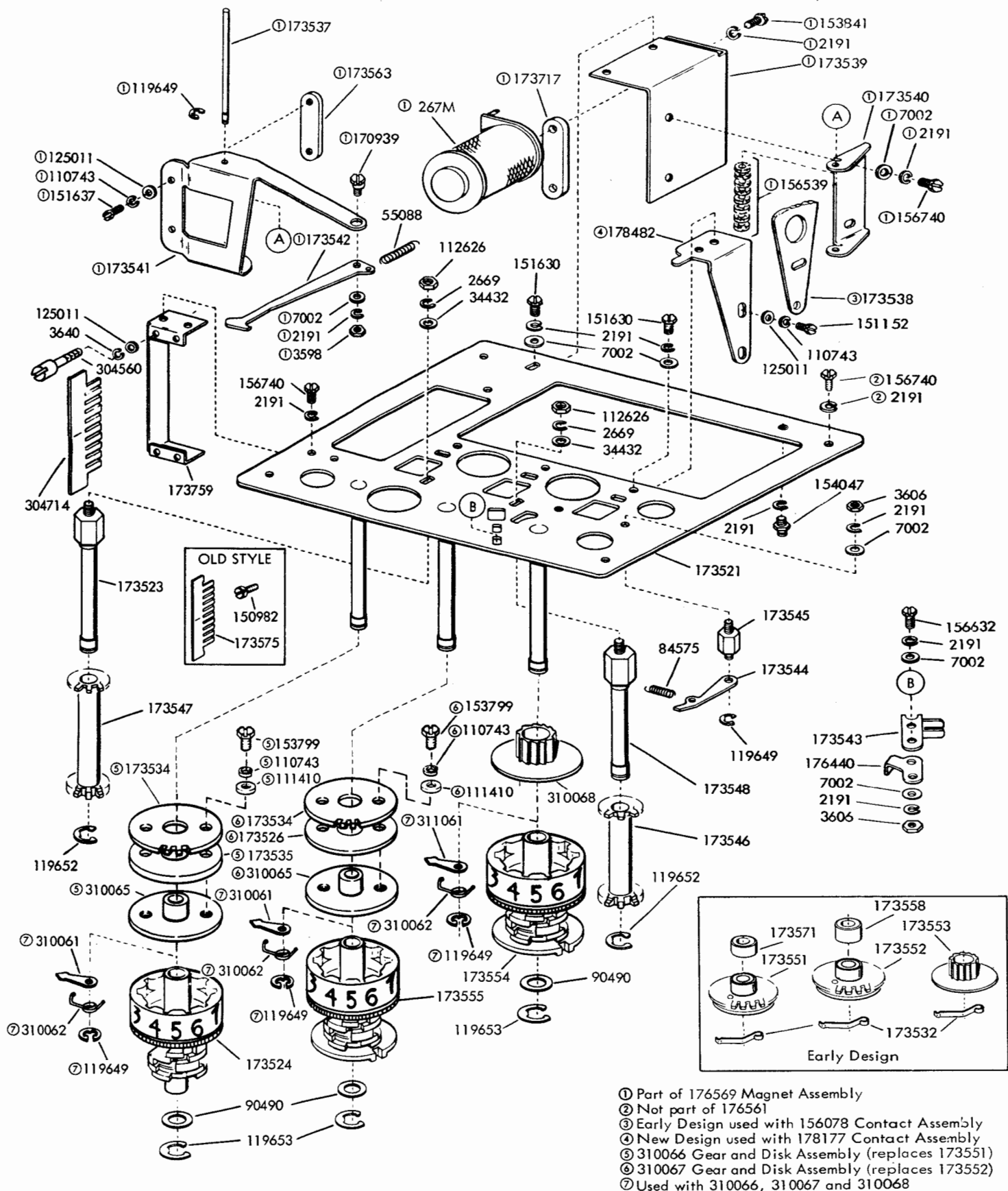
FIGURE 50. 176561 NUMBERING ASSEMBLY (PART OF 176540)
