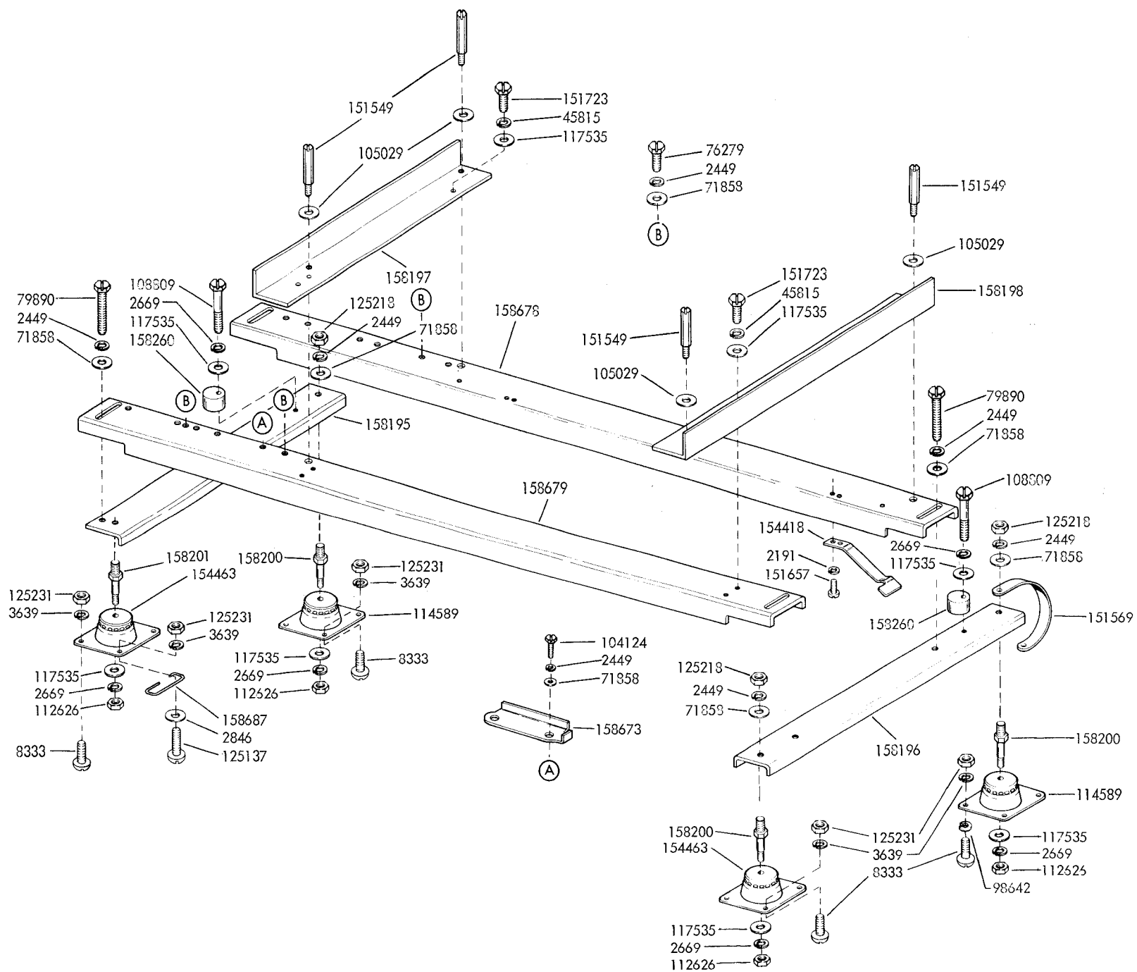
FIGURE 7. CRADLE ASSEMBLY
