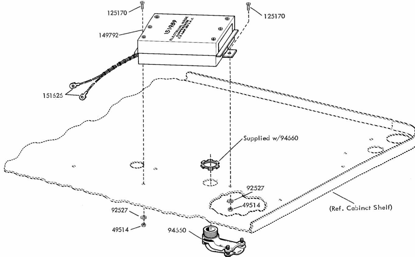
FIGURE 48. 151988 MODIFICATION KIT TO ADD POWER LINE ELECTRICAL NOISE SUPPRESSOR
