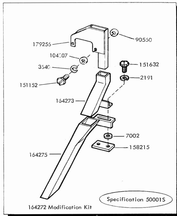
FIGURE 40. 164272 (FOR AUXILIARY REPERFORATOR) AND 170306 (FOR KEYBOARD REPERFORATOR) MODIFICATION KITS TO PROVIDE CHAD DISPOSAL
