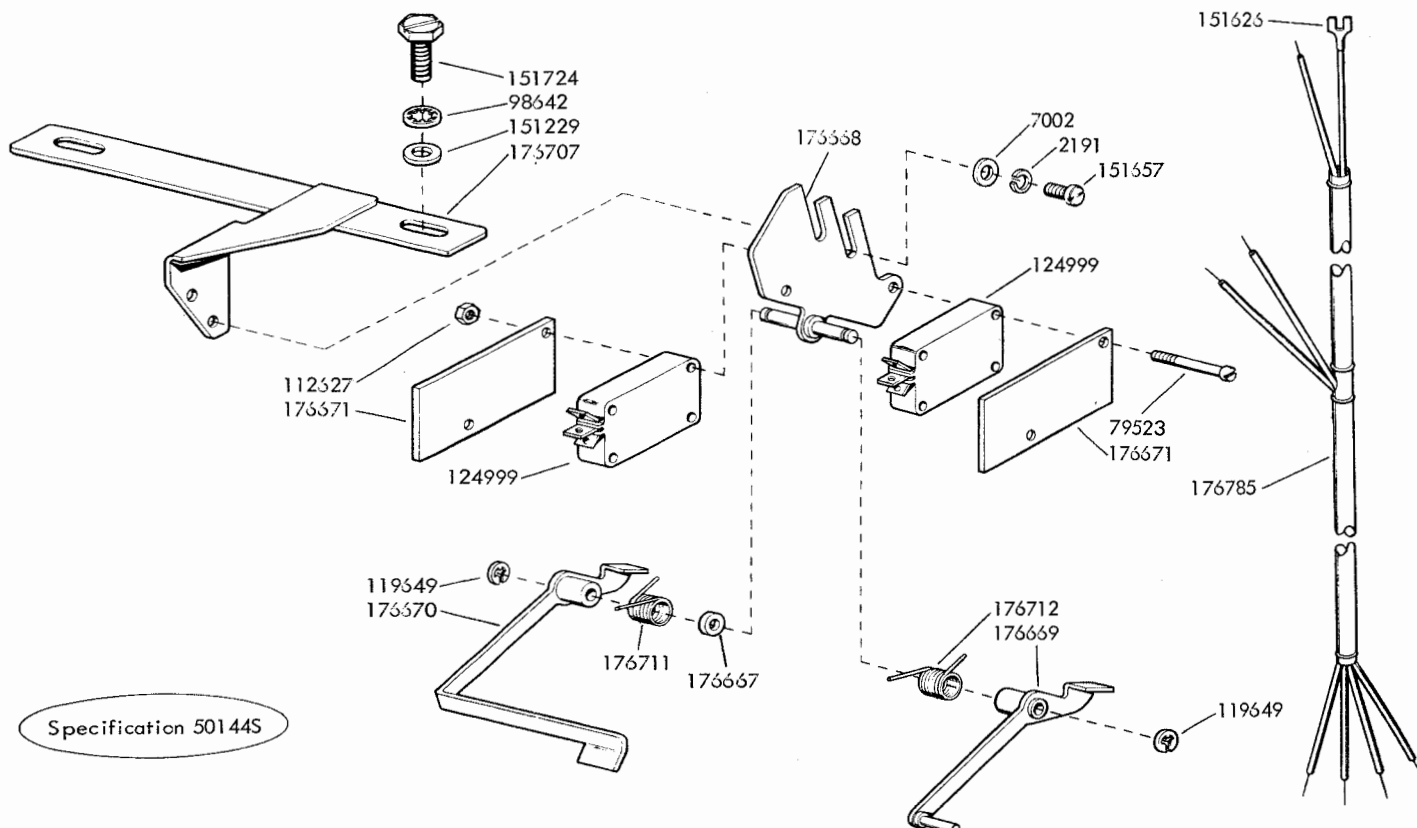
FIGURE 38. 152910** and 179601** MODIFICATION KIT TO ADD DIRECTORY HOLDER OR MESSAGE FILE HOLDER
