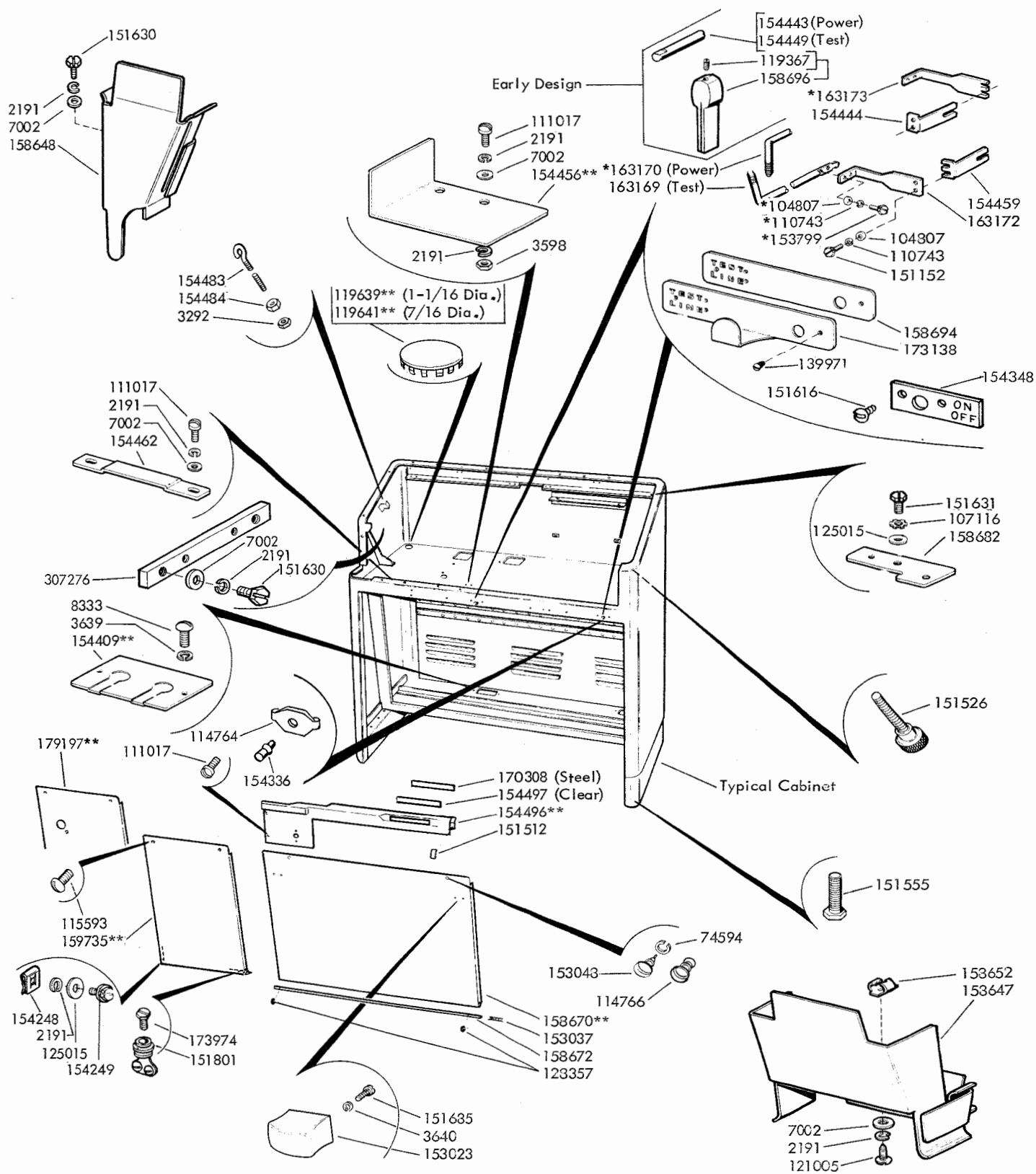
FIGURE 2. CABINET BASE COMMON PARTS
