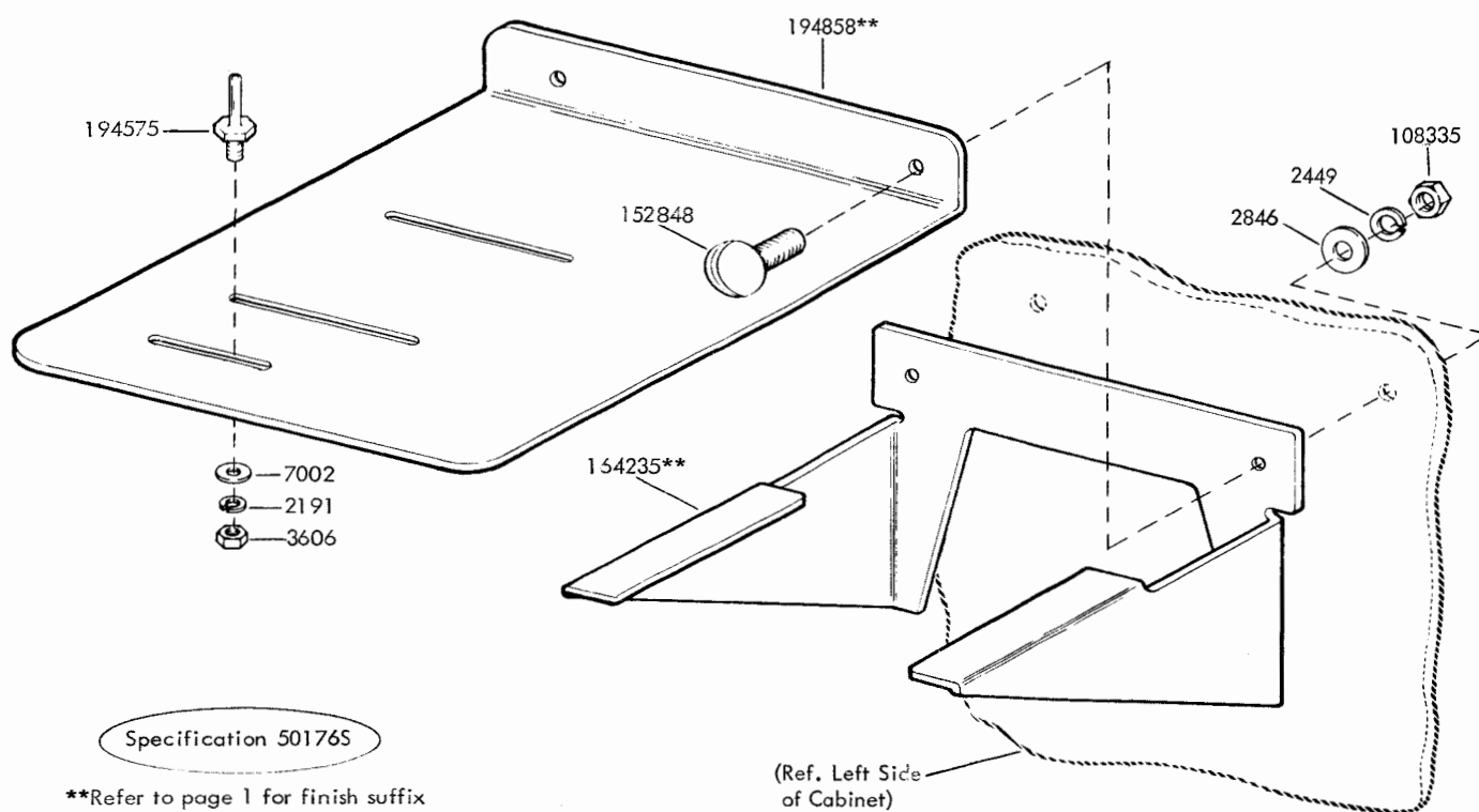
FIGURE 34. 194859** MODIFICATION KIT TO PROVIDE SHELF FOR TAPE WINDER OR TAPE UNWINDER
