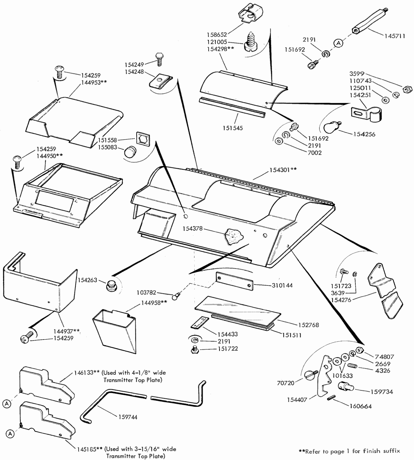
FIGURE 6. CABINET DOME TO ACCOMMODATE PULL-BACK TRANSMITTER
