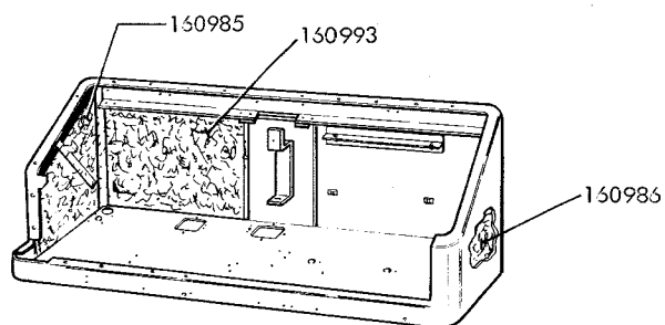
TYPICAL TABLE MODEL CABINET
