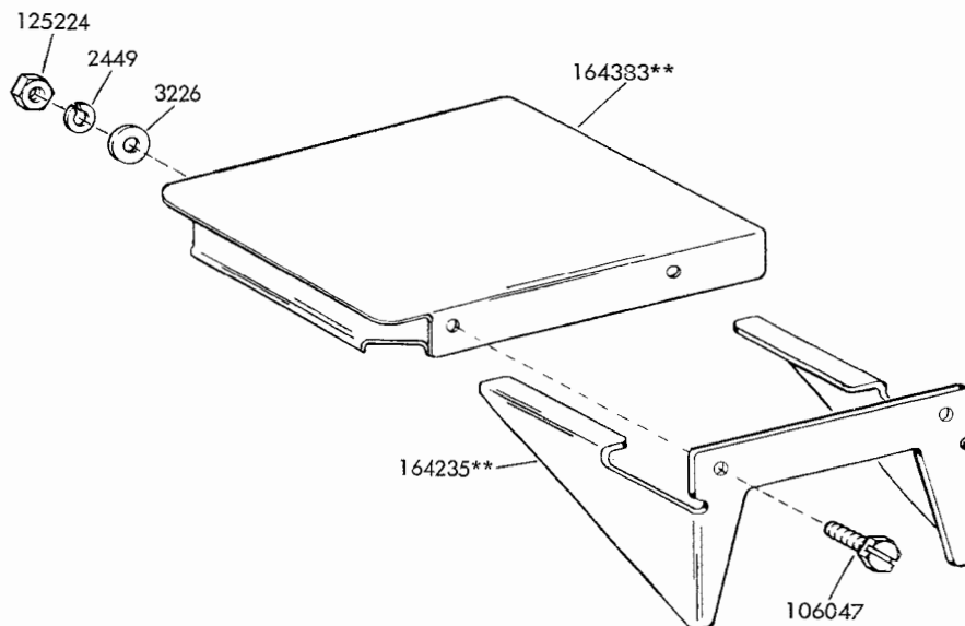
FIGURE 36. 173097** MODIFICATION KIT TO PROVIDE A MOUNTING SHELF FOR LEFT SIDE OF CABINET
