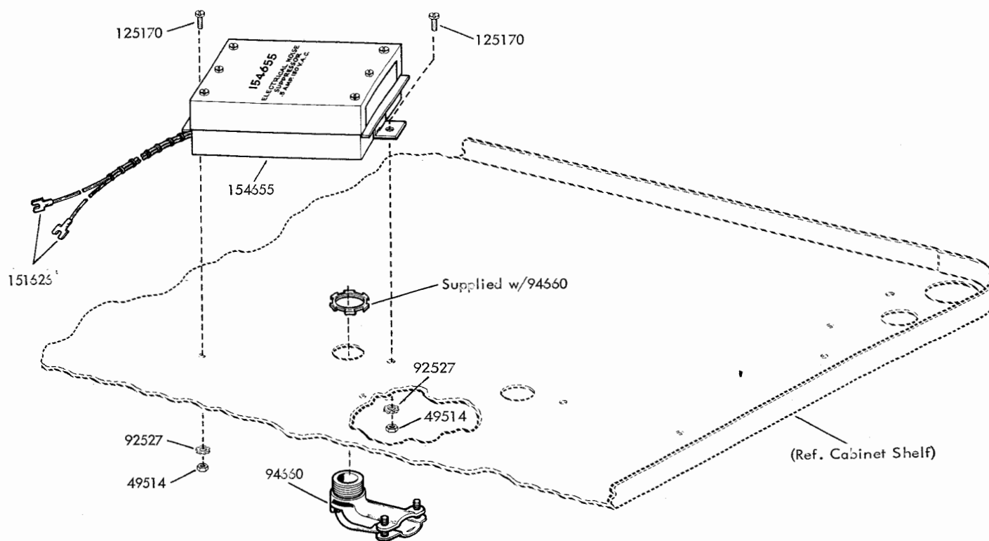
FIGURE 47. 154651 MODIFICATION KIT TO ADD SIGNAL LINE ELECTRICAL NOISE SUPPRESSOR (D. C.)
