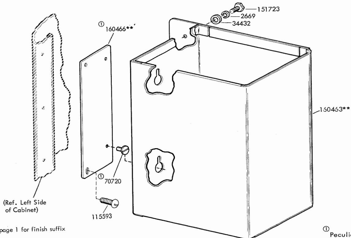
FIGURE 43. 160468** (PIVOTED HEAD TRANSMITTER) AND 160470** (FIXED HEAD TRANSMITTER) MODIFICATION KITS TO PROVIDE TAPE BASKET
