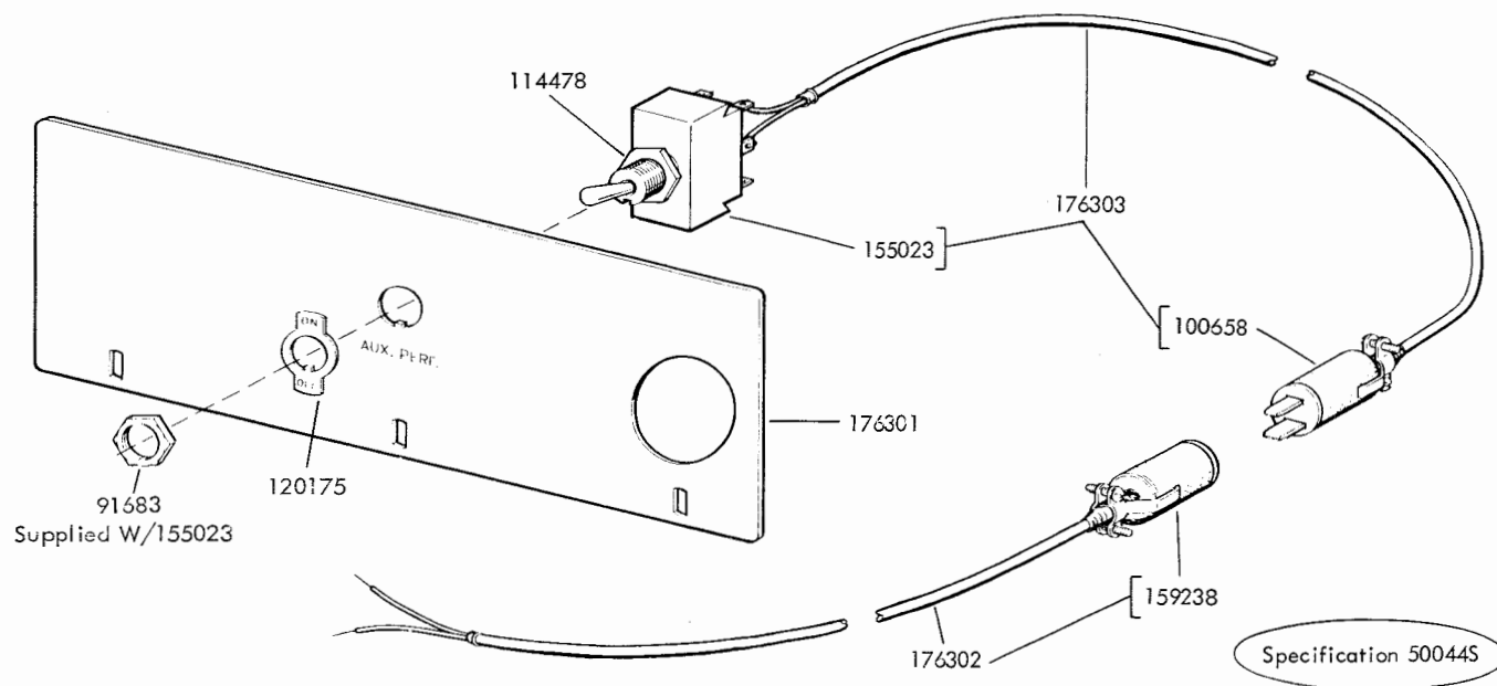
FIGURE 22. 176300 MODIFICATION KIT TO PROVIDE AUXILIARY REPERFORATOR MOTOR CONTROL PANEL
