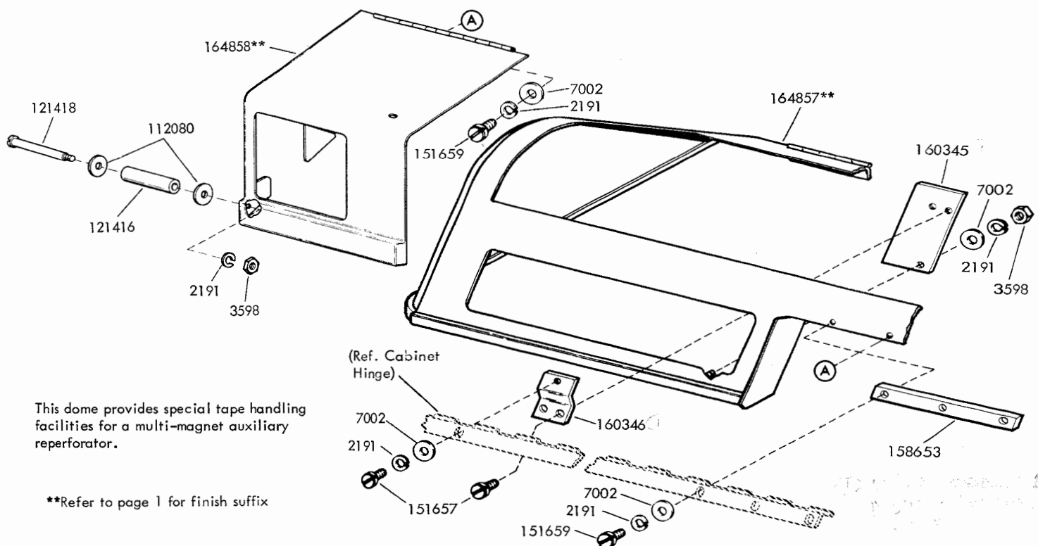
FIGURE 19. CABINET DOME VARIABLE FEATURES
