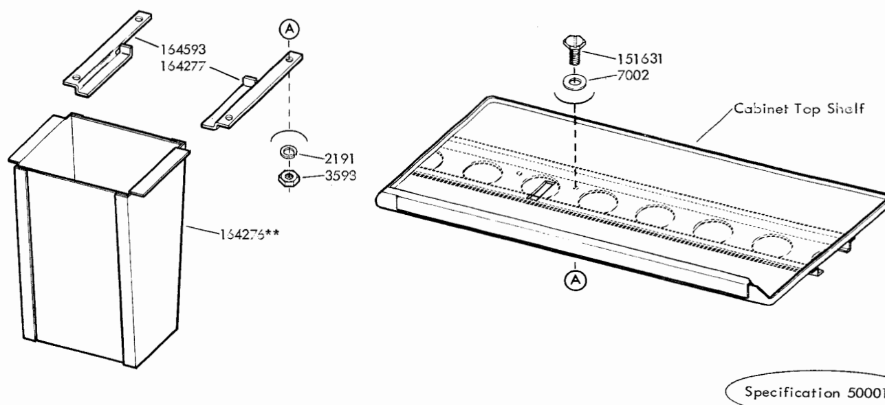
FIGURE 41. 164405** MODIFICATION KIT TO PROVIDE CHAD CONTAINER FOR THE AUXILIARY REPERFORATOR AND/OR KEYBOARD REPERFORATOR
