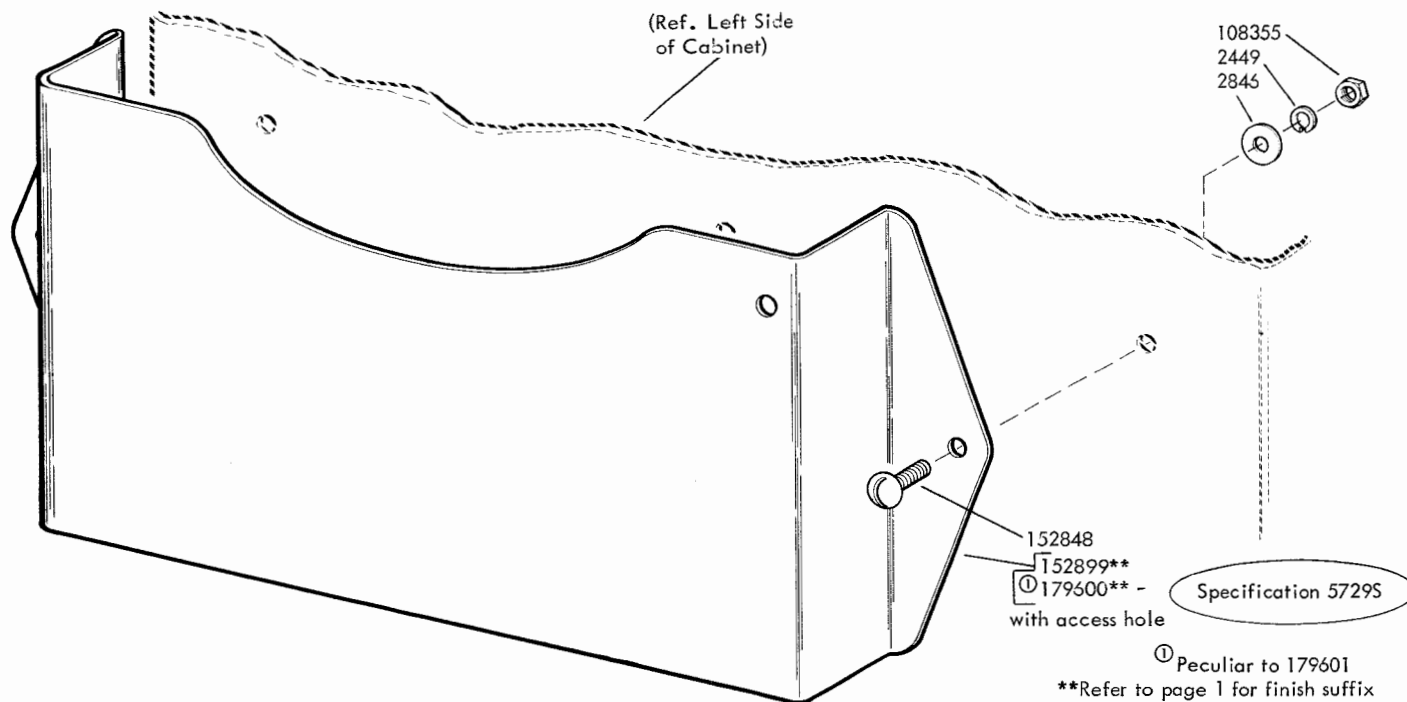
FIGURE 38. 152910** and 179601** MODIFICATION KIT TO ADD DIRECTORY HOLDER OR MESSAGE FILE HOLDER
