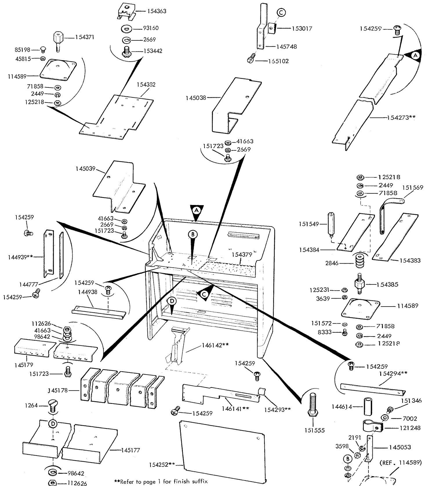
FIGURE 4. CABINET BASE TO ACCOMMODATE PULL-BACK TRANSMITTER
