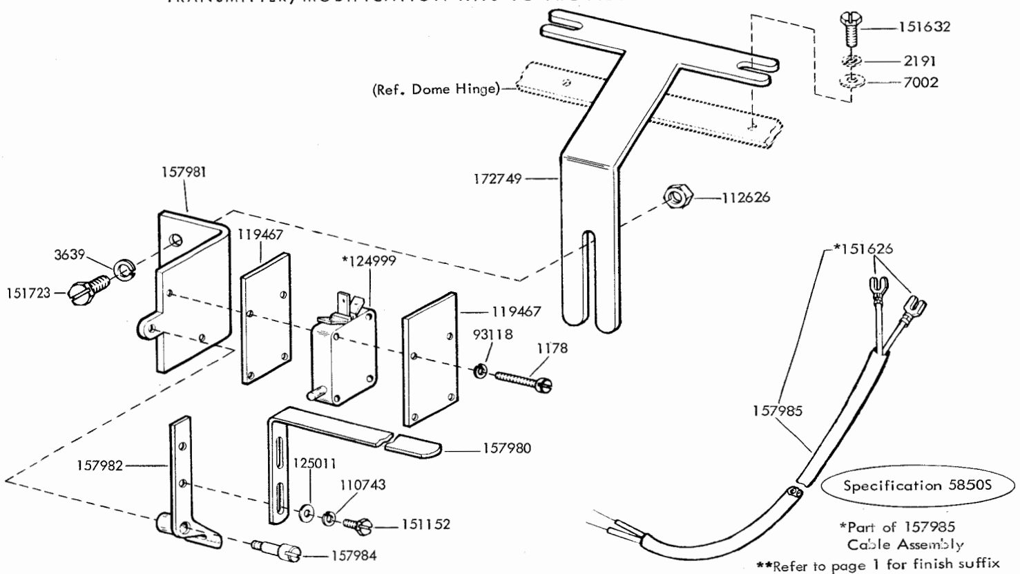
FIGURE 44. 154756 MODIFICATION KIT TO PROVIDE FORM-OUT ALARM
