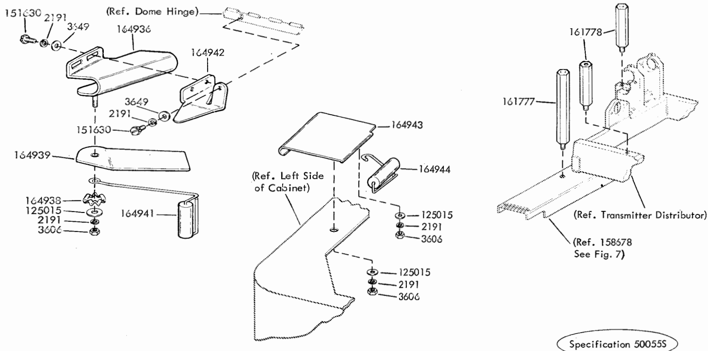
FIGURE 45. 193675 MODIFICATION KIT TO PROVIDE CABINET WITH TWO HINGED PANELS IN LOWER CAVITY
