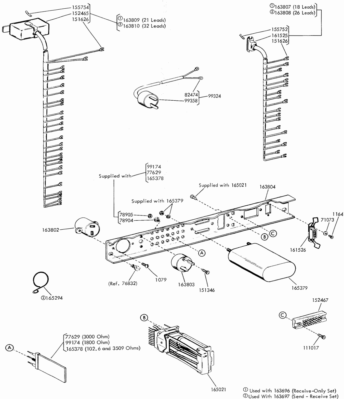
FIGURE 16. 163696 AND 163697 RELAY PANEL ASSEMBLIES
