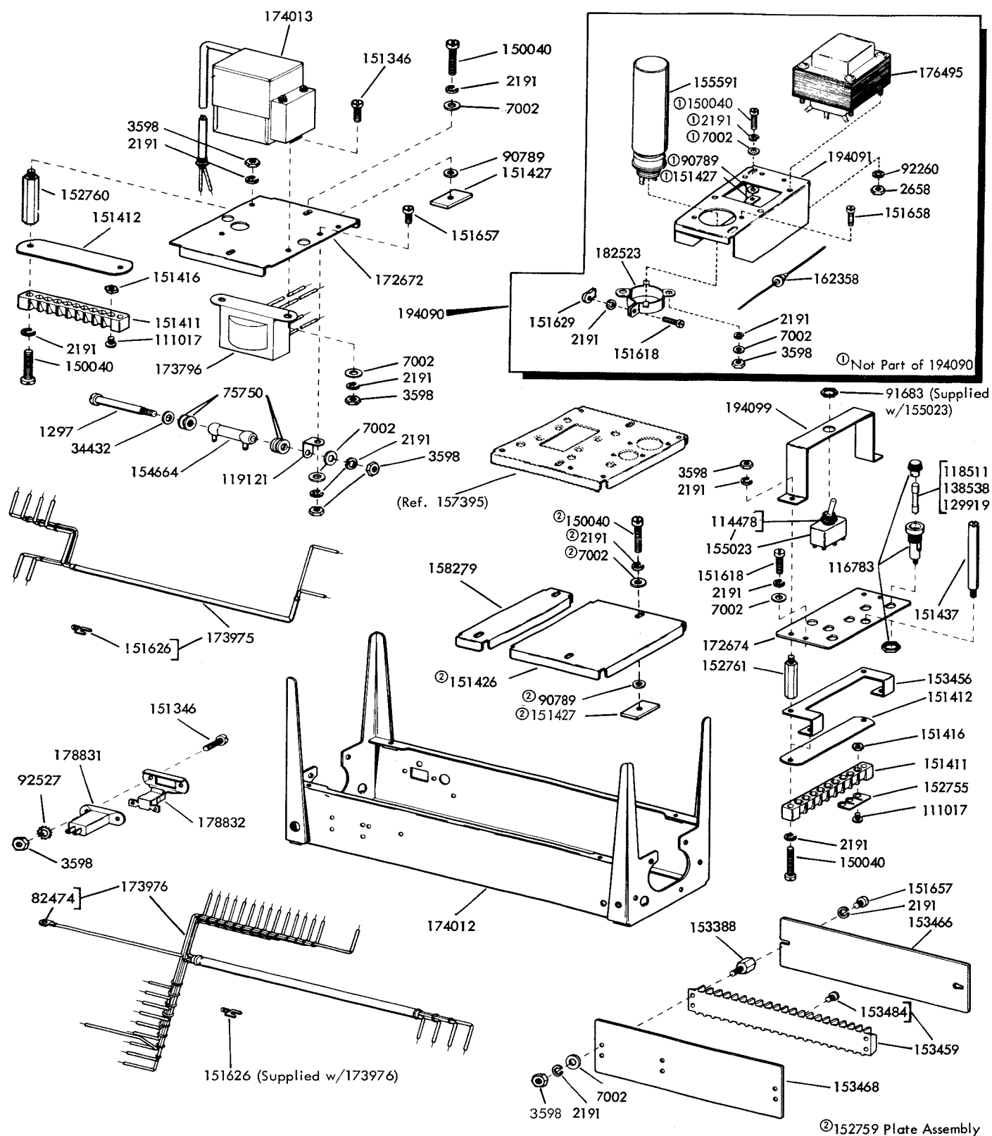
FIGURE 4. COMPONENTS FOR UNIT WITH ELECTRICAL NOISE SUPPRESSOR AND FILAMENT TRANSFORMER
