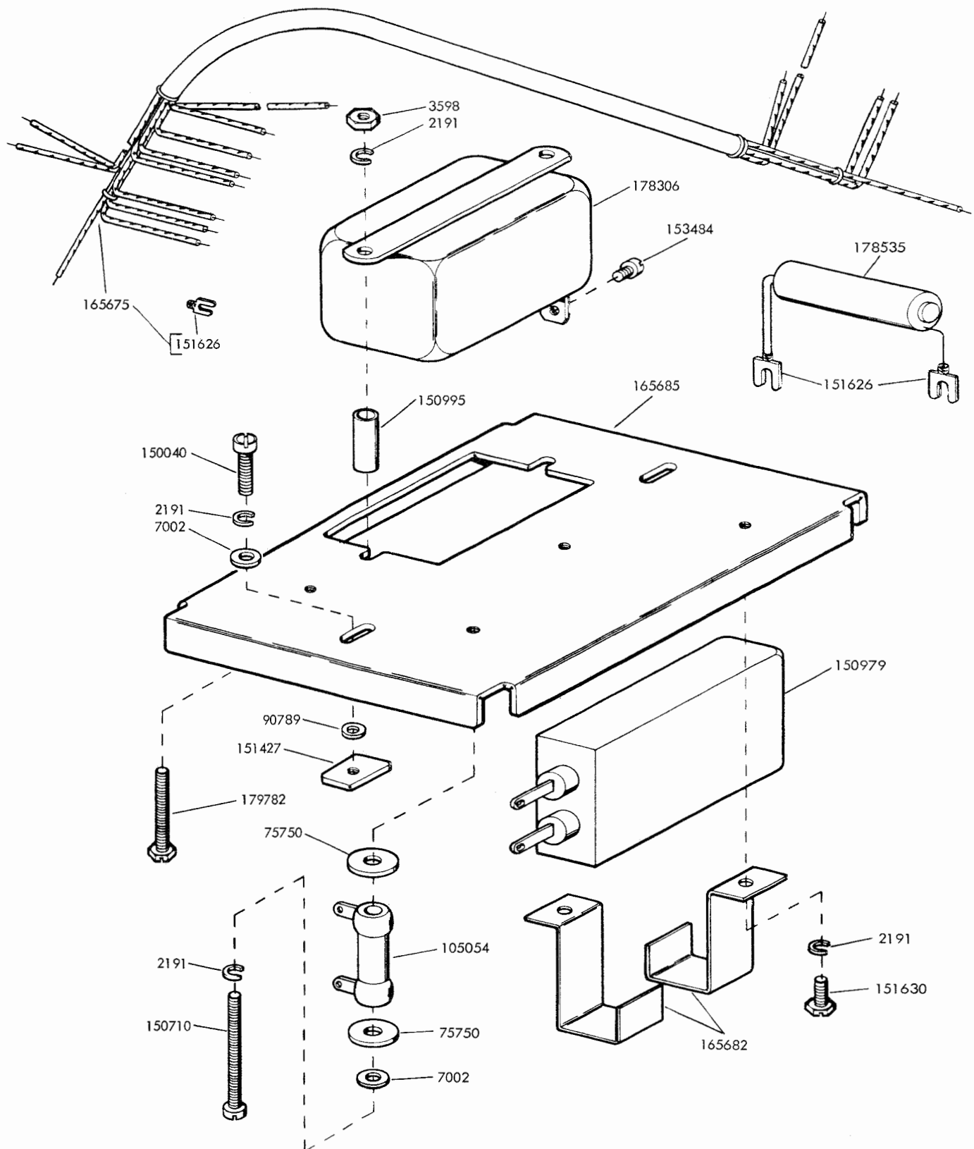
FIGURE 19. 165687 MOTOR CONTROL RELAY ASSEMBLY
