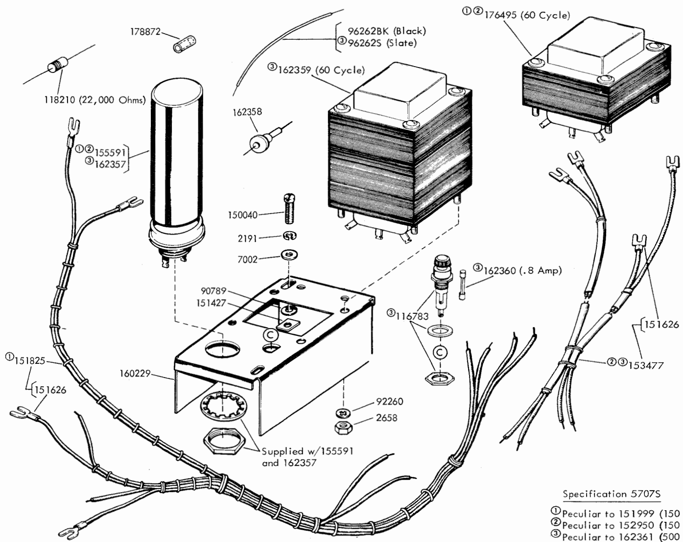
FIGURE 8. 151999, 152950 AND 162361 RECTIFIER AND CABLE ASSEMBLIES
