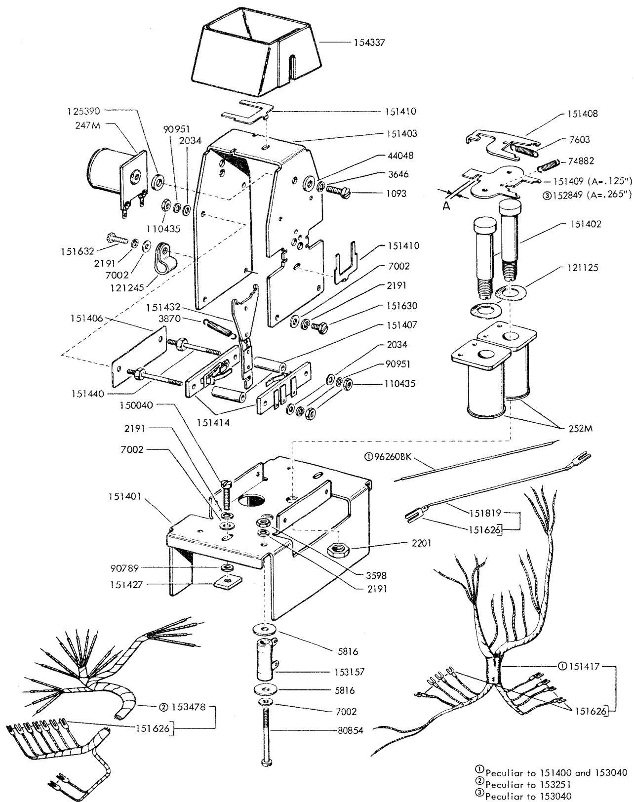
FIGURE 18. 151400, 153040 AND 153251 MOTOR CONTROL ASSEMBLIES
