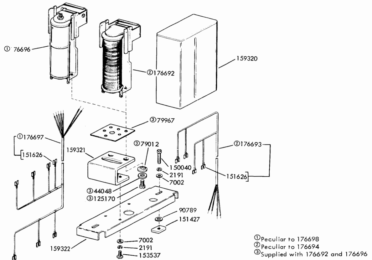
FIGURE 23. 176810 ANSWER-BACK CONTROL RELAY ASSEMBLY
