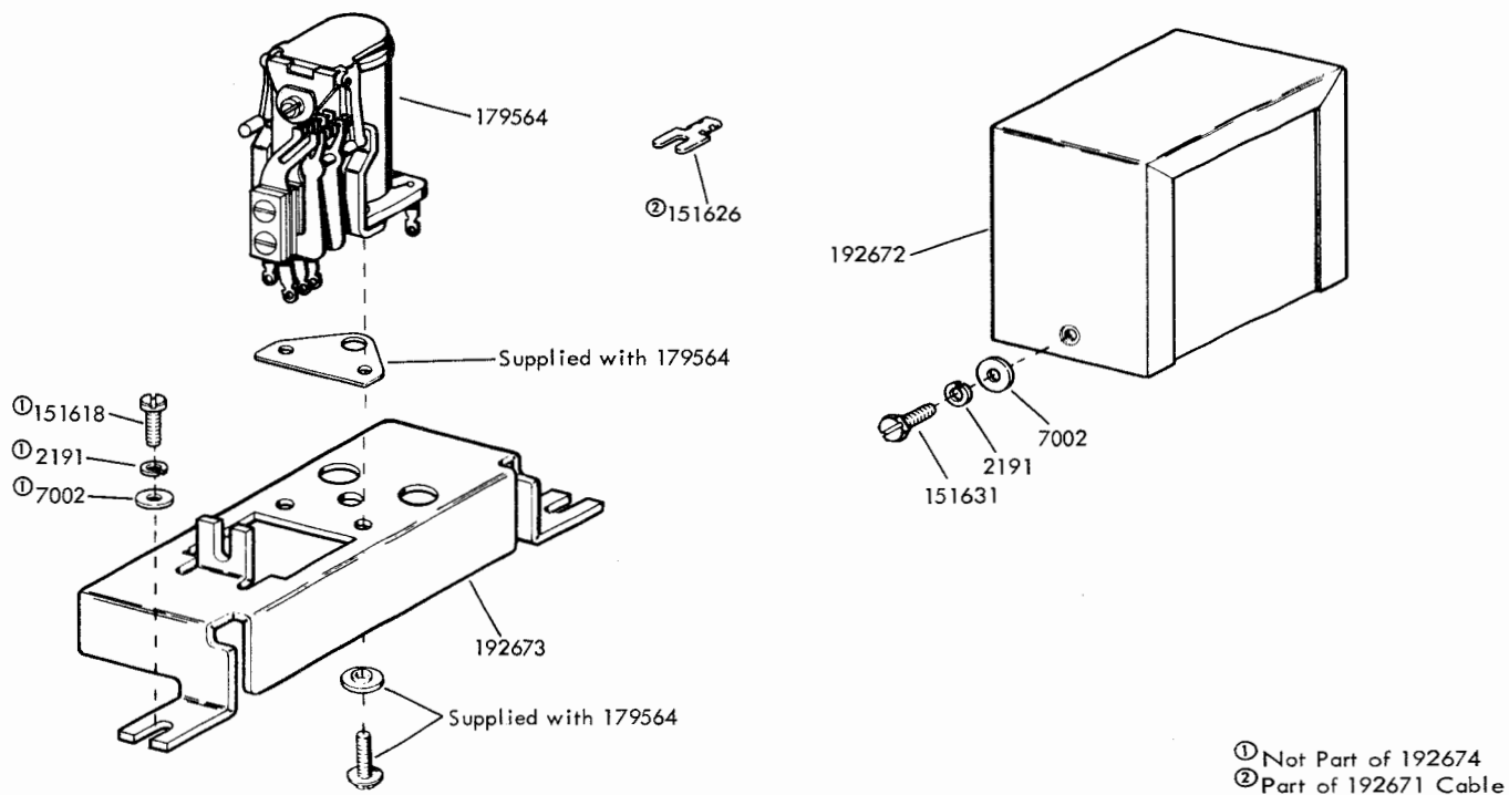
FIGURE 6. 192674 RELAY ASSEMBLY
