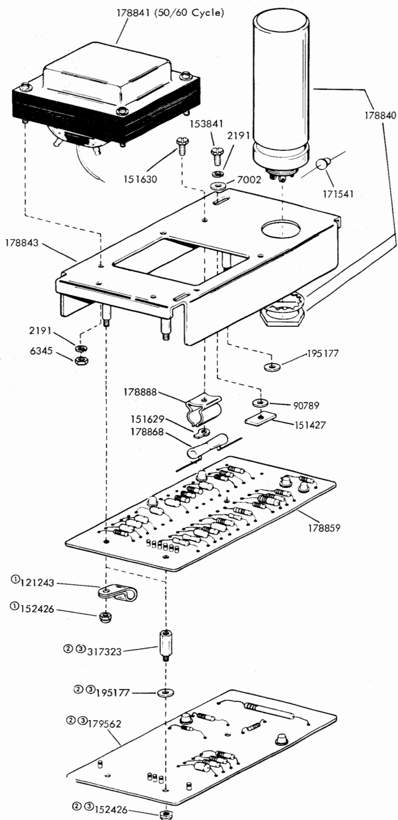
FIGURE 9. 177010, 192669 AND 194369 SELECTOR MAGNET DRIVER ASSEMBLIES (WITH OPEN LINE DETECTOR)
