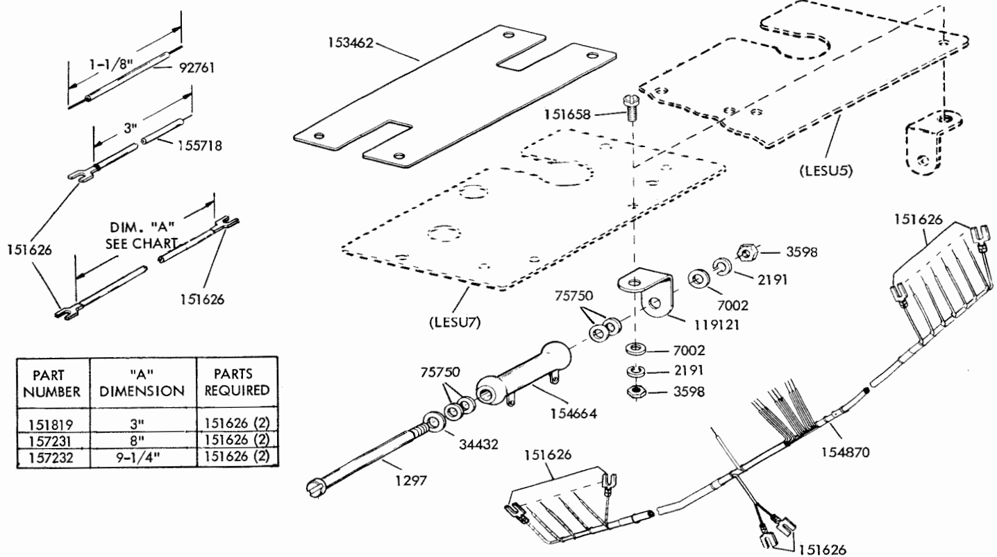
FIGURE 31. LINE SHUNT RELAY (NEW STYLE)
