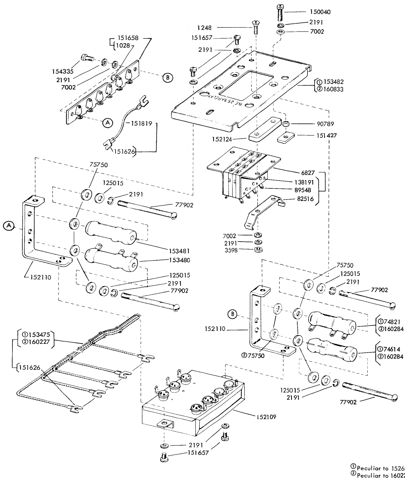
FIGURE 11. 152623 AND 160226 LINE RELAY MOUNTING ASSEMBLIES
