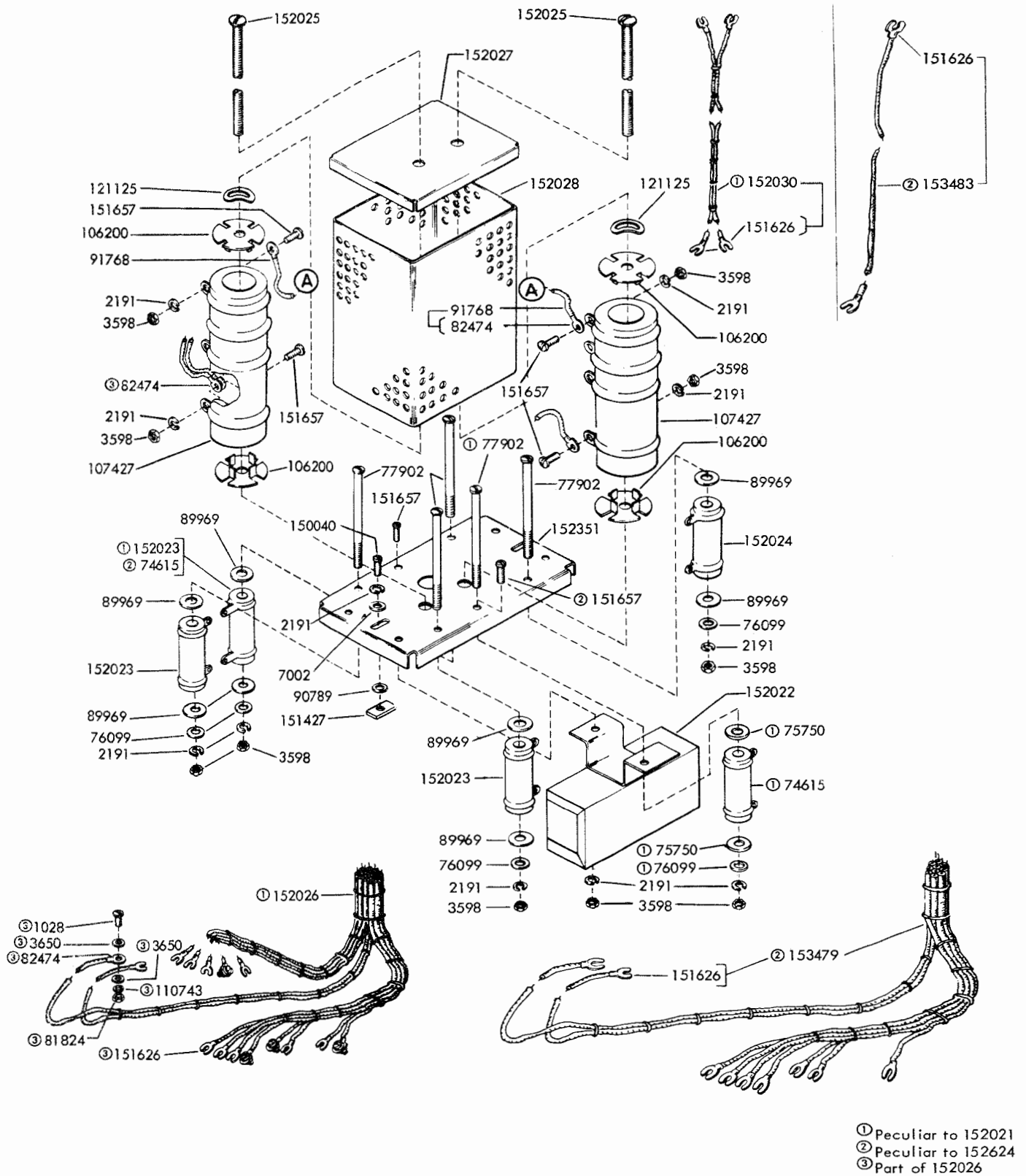
FIGURE 17. 152021 AND 152624 CAPACITOR-RESISTOR ASSEMBLIES
