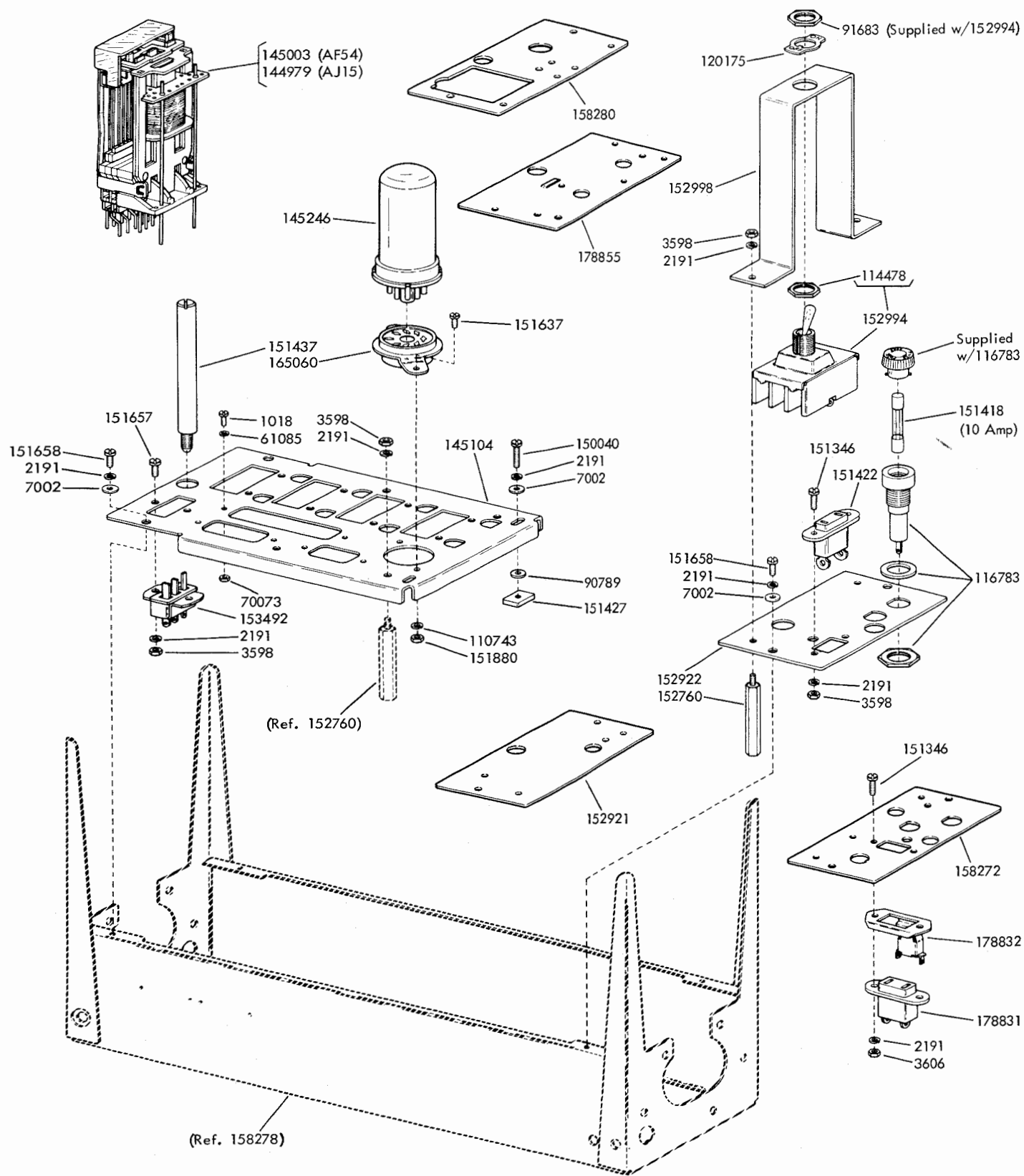
FIGURE 2. MOUNTING PLATES AND COMPONENTS
