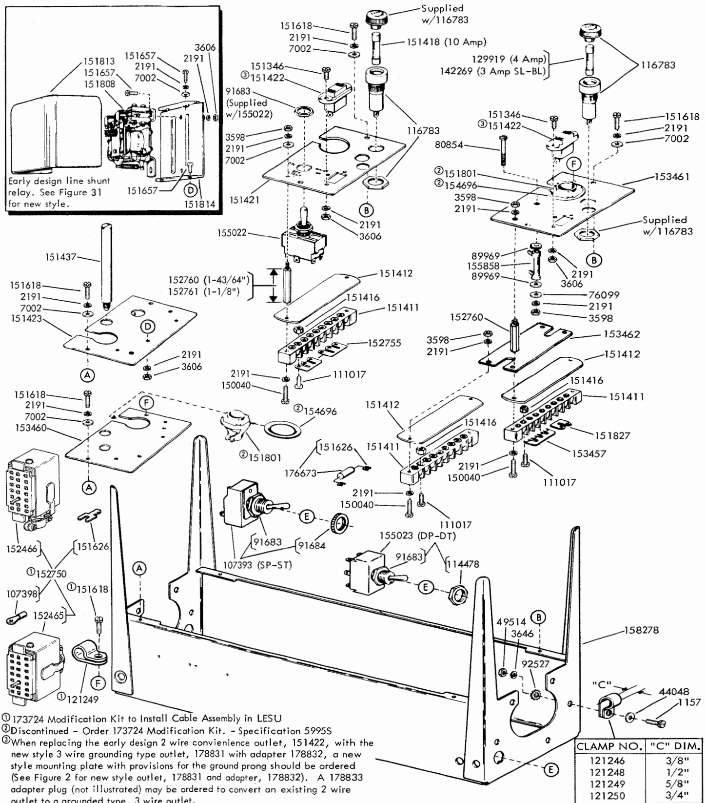
FIGURE 1. CONTAINER WITH MOUNTING PLATES AND COMPONENTS
