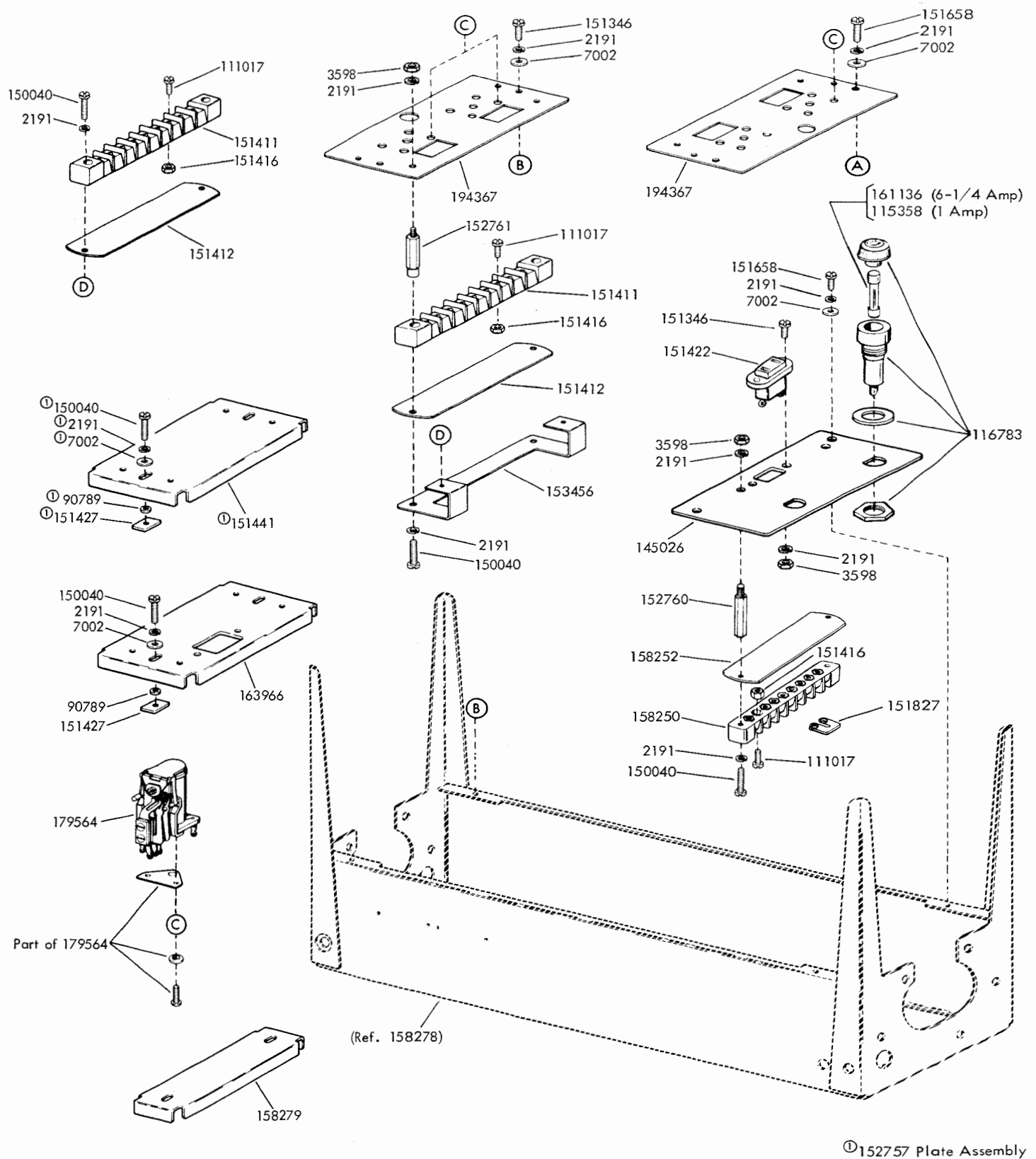
FIGURE 3. MOUNTING PLATES AND COMPONENTS (Continued)
