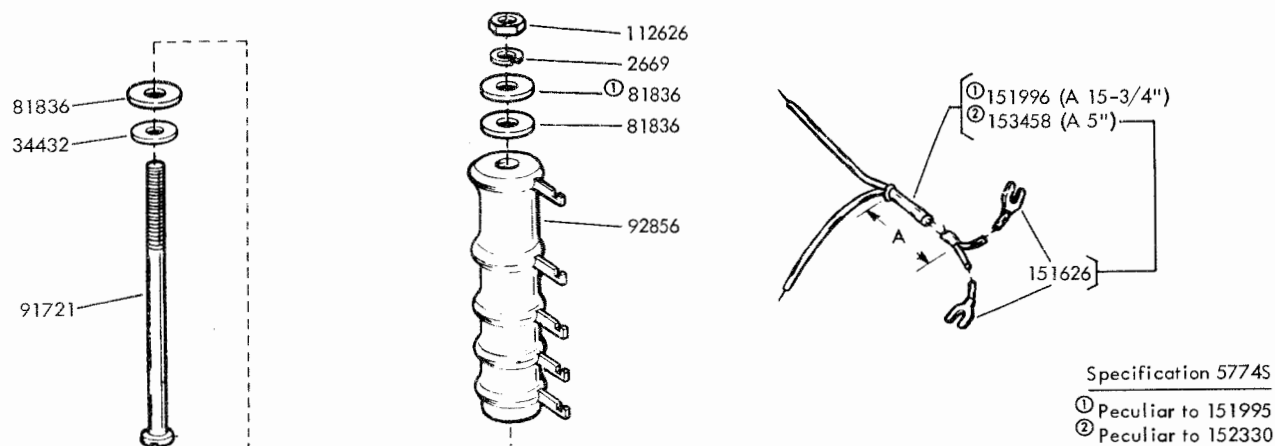
FIGURE 29. 159397 MODIFICATION KIT TO CONVERT THE 152623 LINE RELAY MOUNTING ASSEMBLY TO THE 160226 ASSEMBLY
