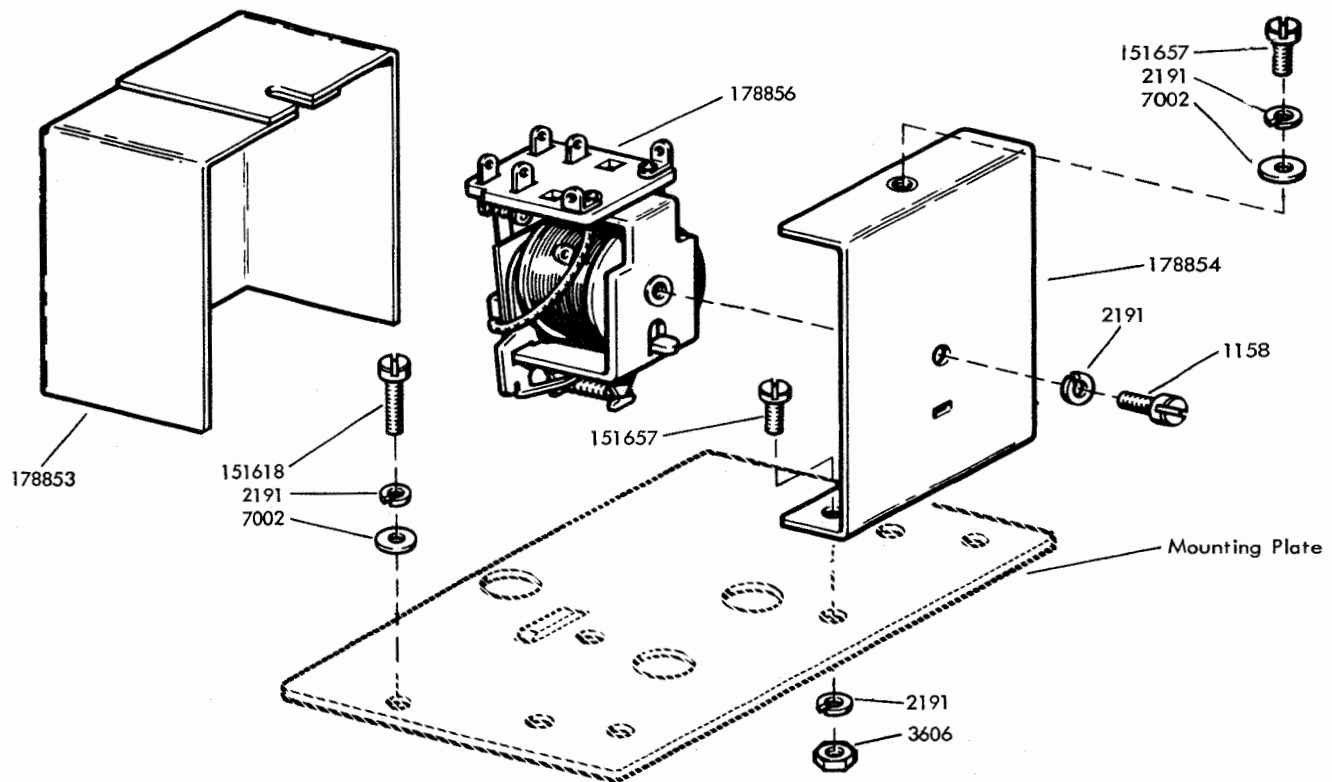
FIGURE 31. LINE SHUNT RELAY (NEW STYLE)
