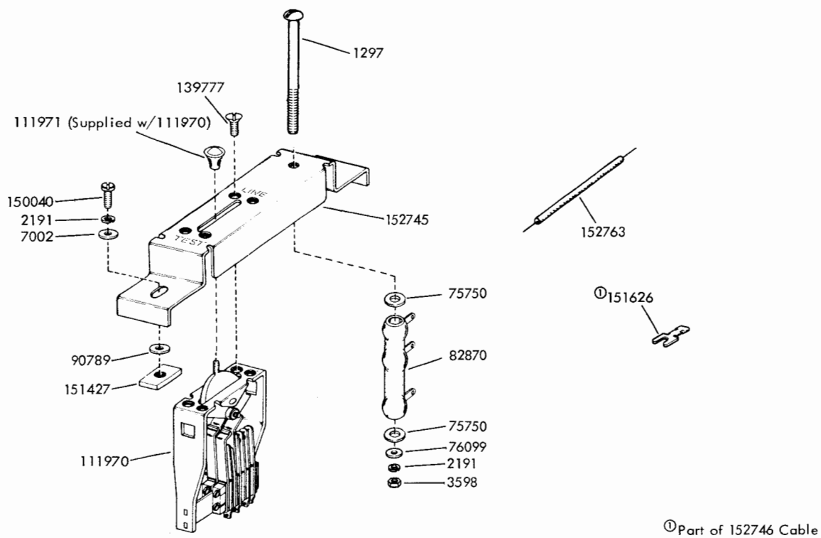
FIGURE 14. 152744 LINE TEST KEY ASSEMBLY
