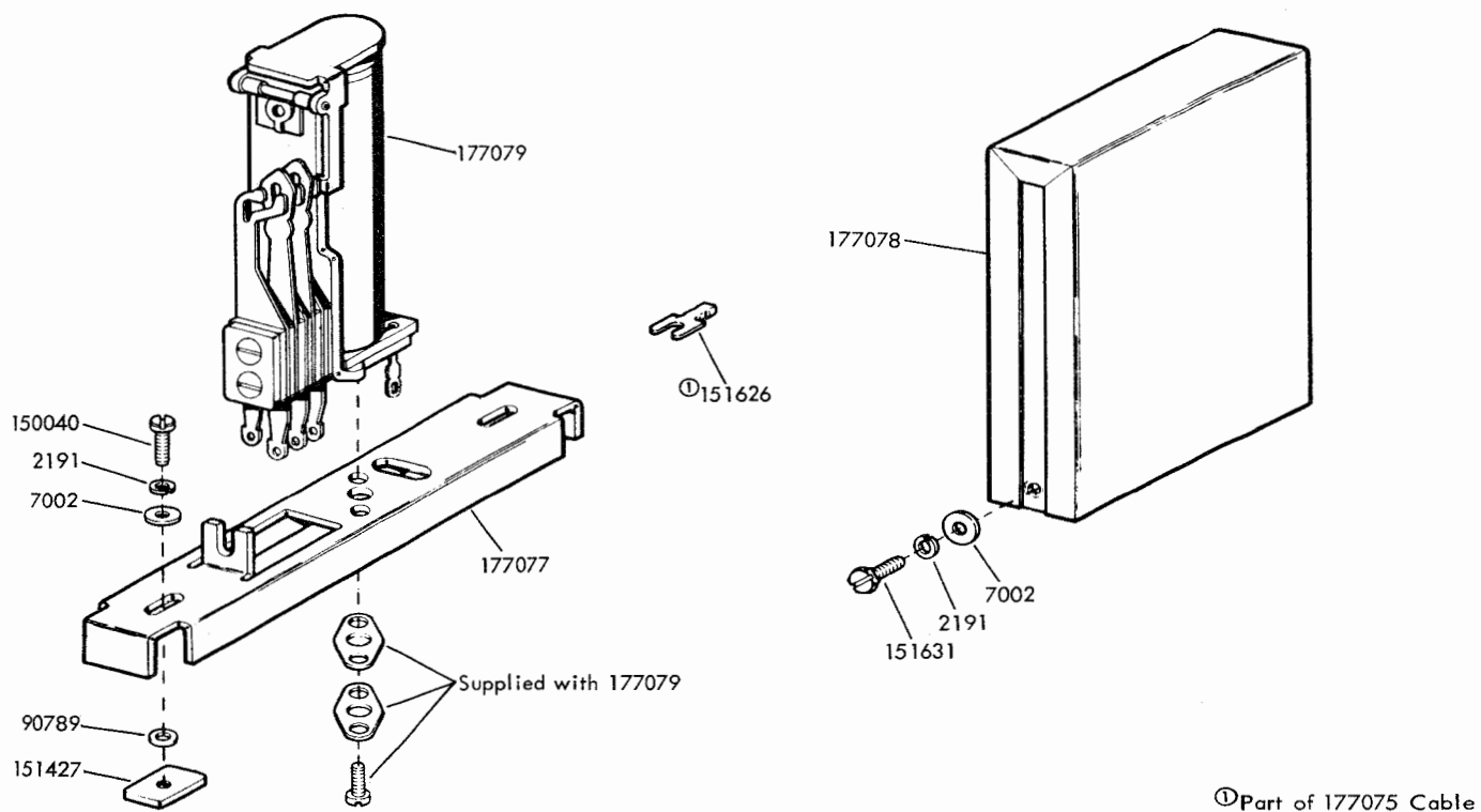
FIGURE 5. 177076 RELAY ASSEMBLY
