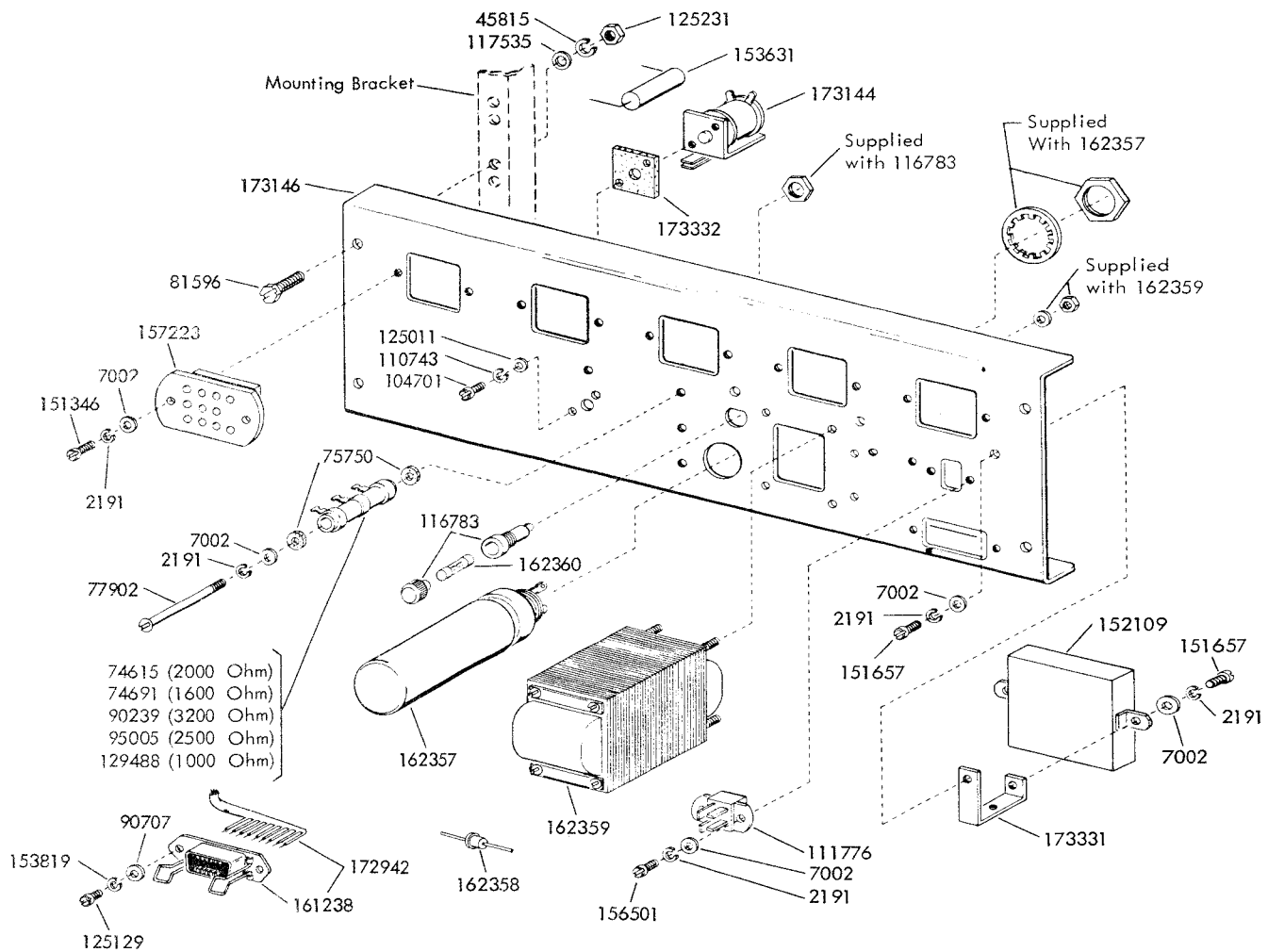
FIGURE 26. 164271 ELECTRICAL SERVICE ASSEMBLY
