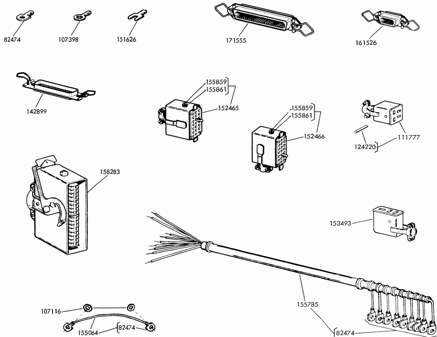
FIGURE 34. CABLE COMPONENTS
