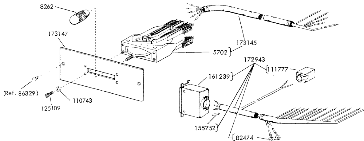
FIGURE 26. 164271 ELECTRICAL SERVICE ASSEMBLY
