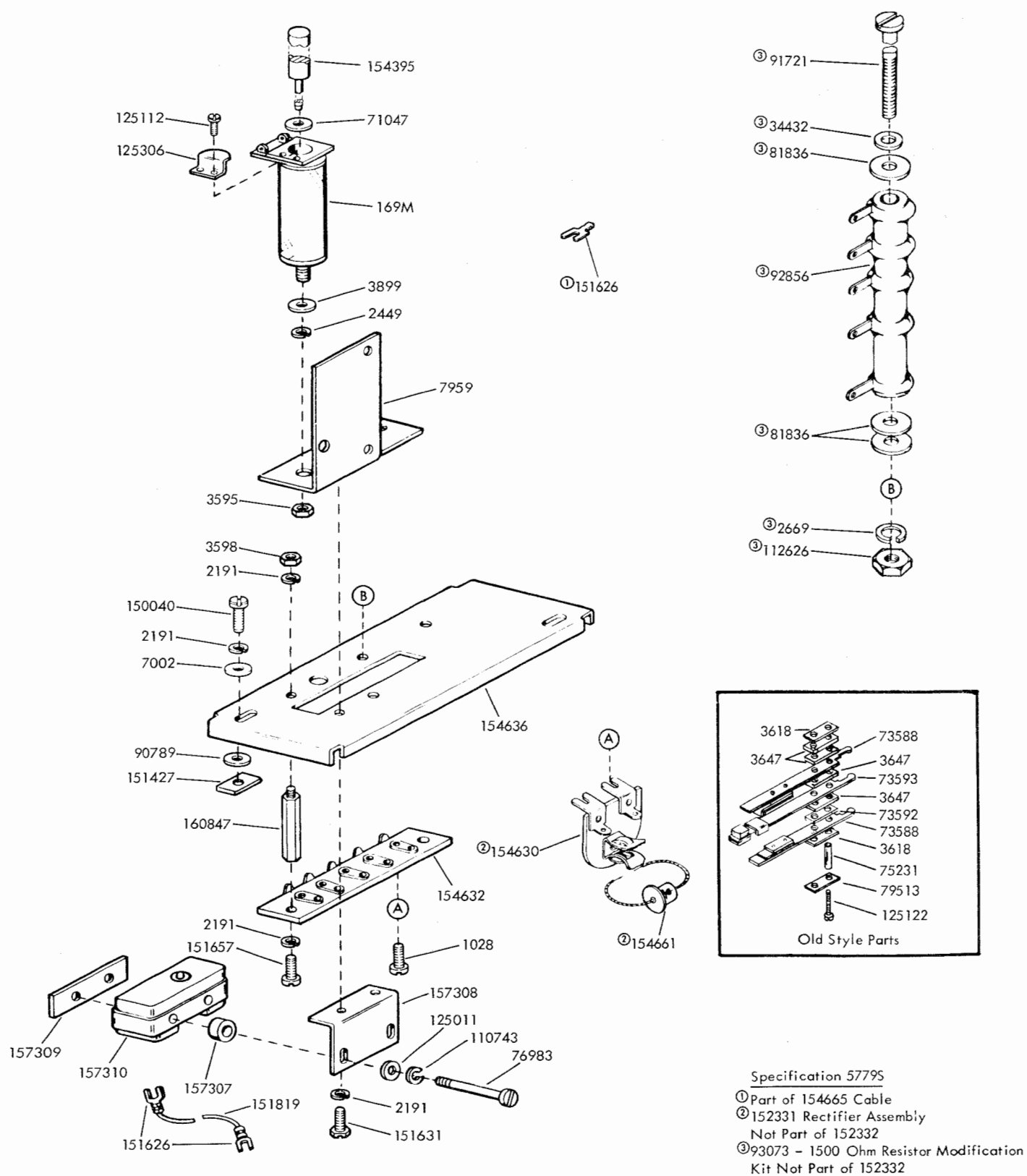
FIGURE 20. 152332 MOTOR CONTROL RELAY ASSEMBLY
