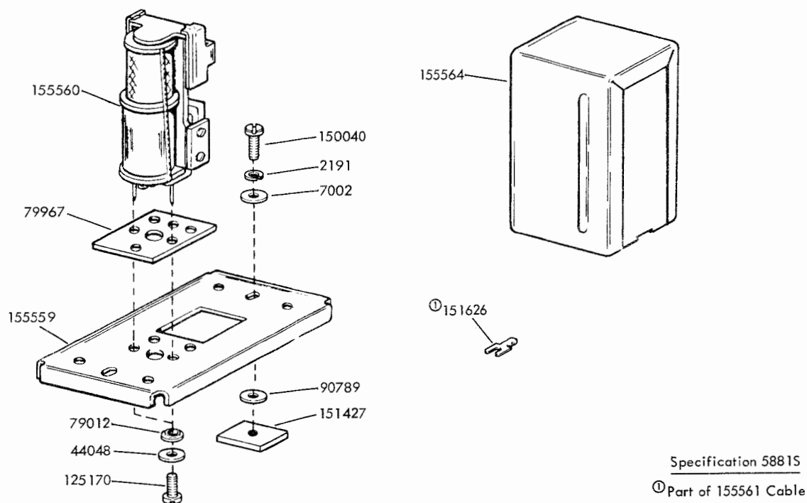
FIGURE 28. 155558 DC CONTROL RELAY ASSEMBLY
