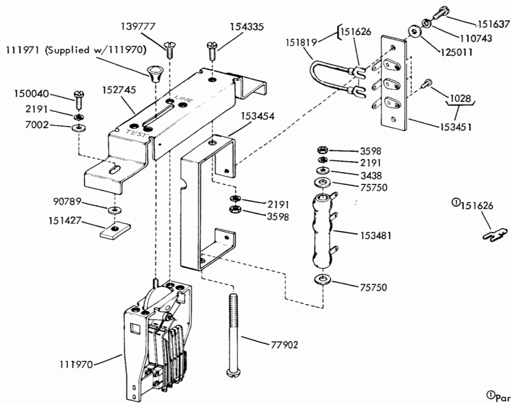
FIGURE 13. 152625 LINE TEST KEY ASSEMBLY
