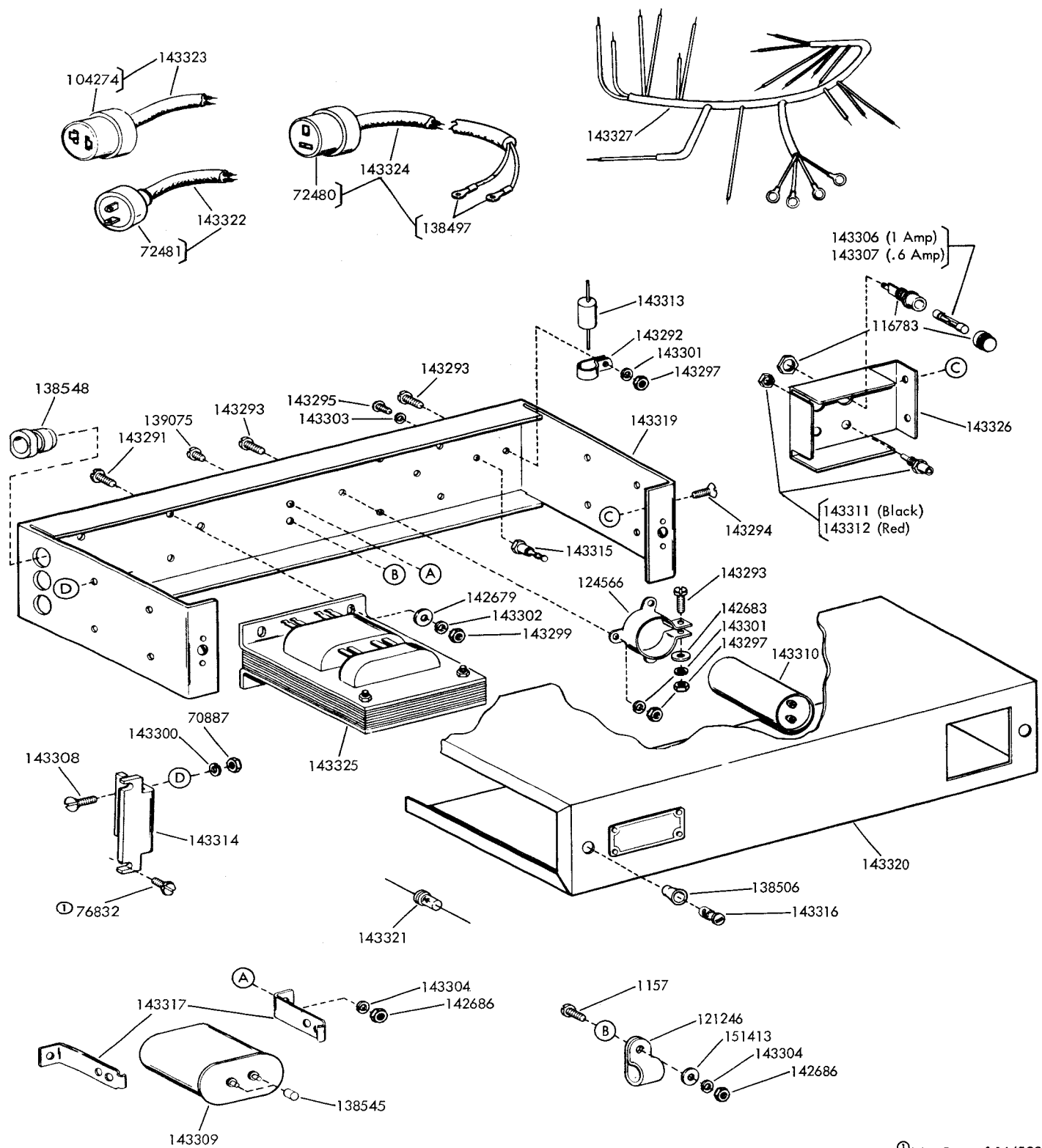
FIGURE 7. 164503 RECTIFIER ASSEMBLY
