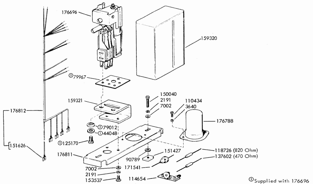
FIGURE 23. 176810 ANSWER-BACK CONTROL RELAY ASSEMBLY
